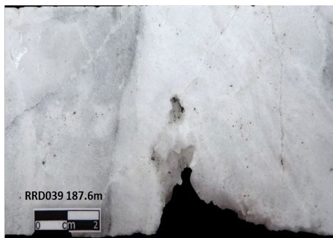
Figure 4: Photos of core specimens from the Susi vein drill hole RRD037(left) and the Pertama vein drillhole RRD039 (right). RRD037-190.9m is a milled and cemented fault breccia with rounded fragments of quartz and argillic altered volcanic. Part of a 1m wide sample interval that assayed 8.09g/t Au, 17.8g/t Ag (8.3g/t AuEq) from 190-191m. RRD039-187.6 is crystalline quartz with faint, fine bands of glassy quartz. Part of a 0.7m wide sample interval that assayed 2.75g/t Au, 55g/t Ag (3.41g/t AuEq) from 187-187.7m.
