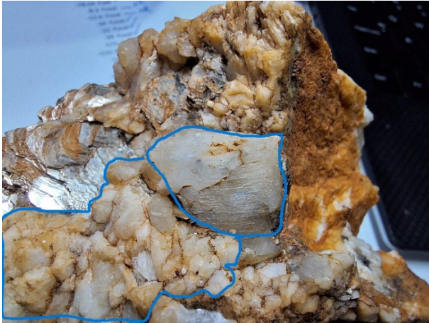
Figure 3. Spodumene crystals (blue outlines) identified by crystal shape, striated surface and orange-tan glow under 365nm UV light (Figure 3A). The visually estimated spodumene content is approximately 5-10%, Quartz 40-50%, Feldspar 20-30% and Mica 5-10%. Sample collected from the same location and rock unit sampled in this announcement were collected. 3 .
