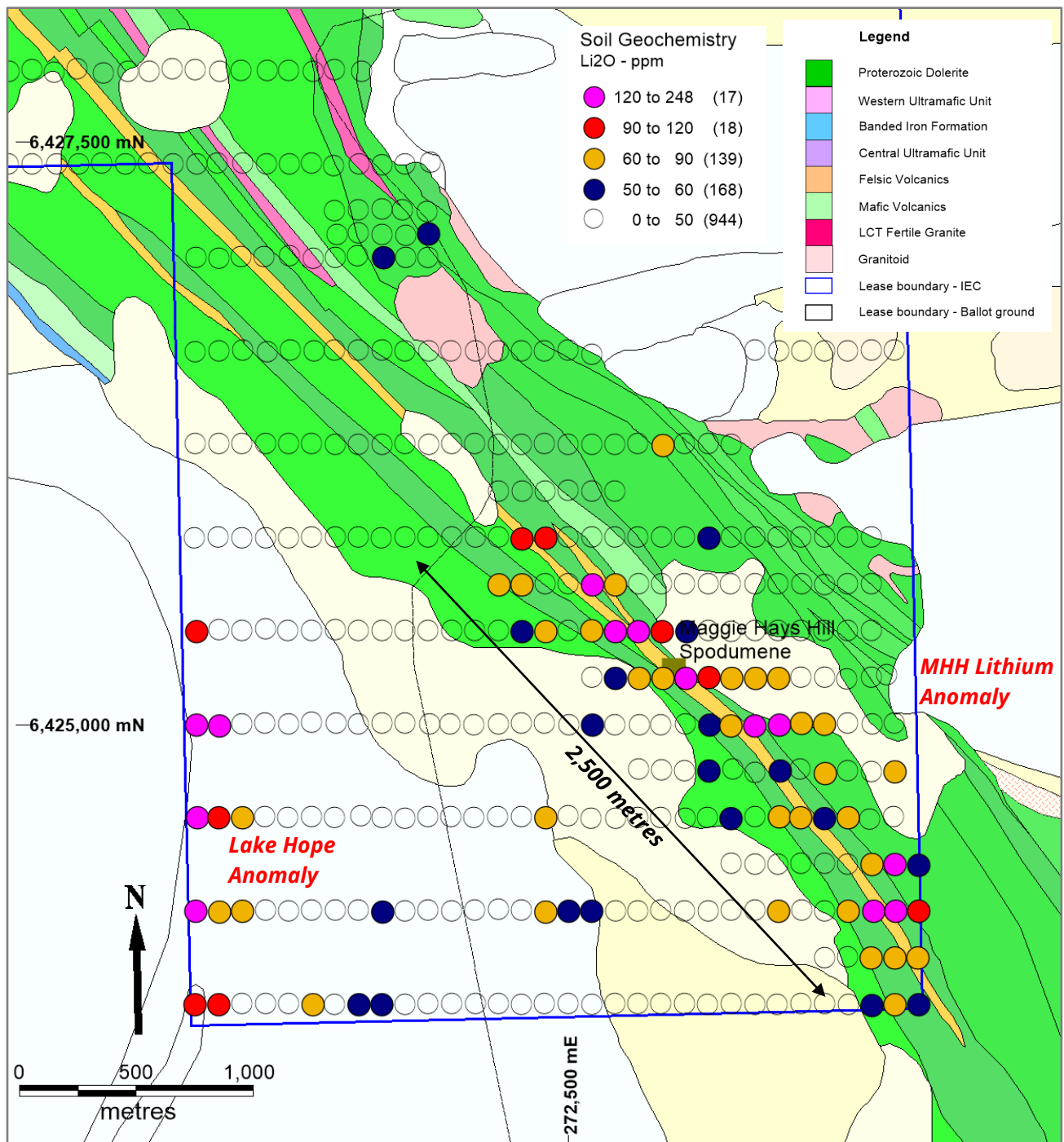
Figure 5. Southern end of tenement E63/2039 highlighting the strong association between lithium - tantalum assay results and mapped outcropping pegmatites covering 2,500 metres of strike at the MHH lithium anomaly.
