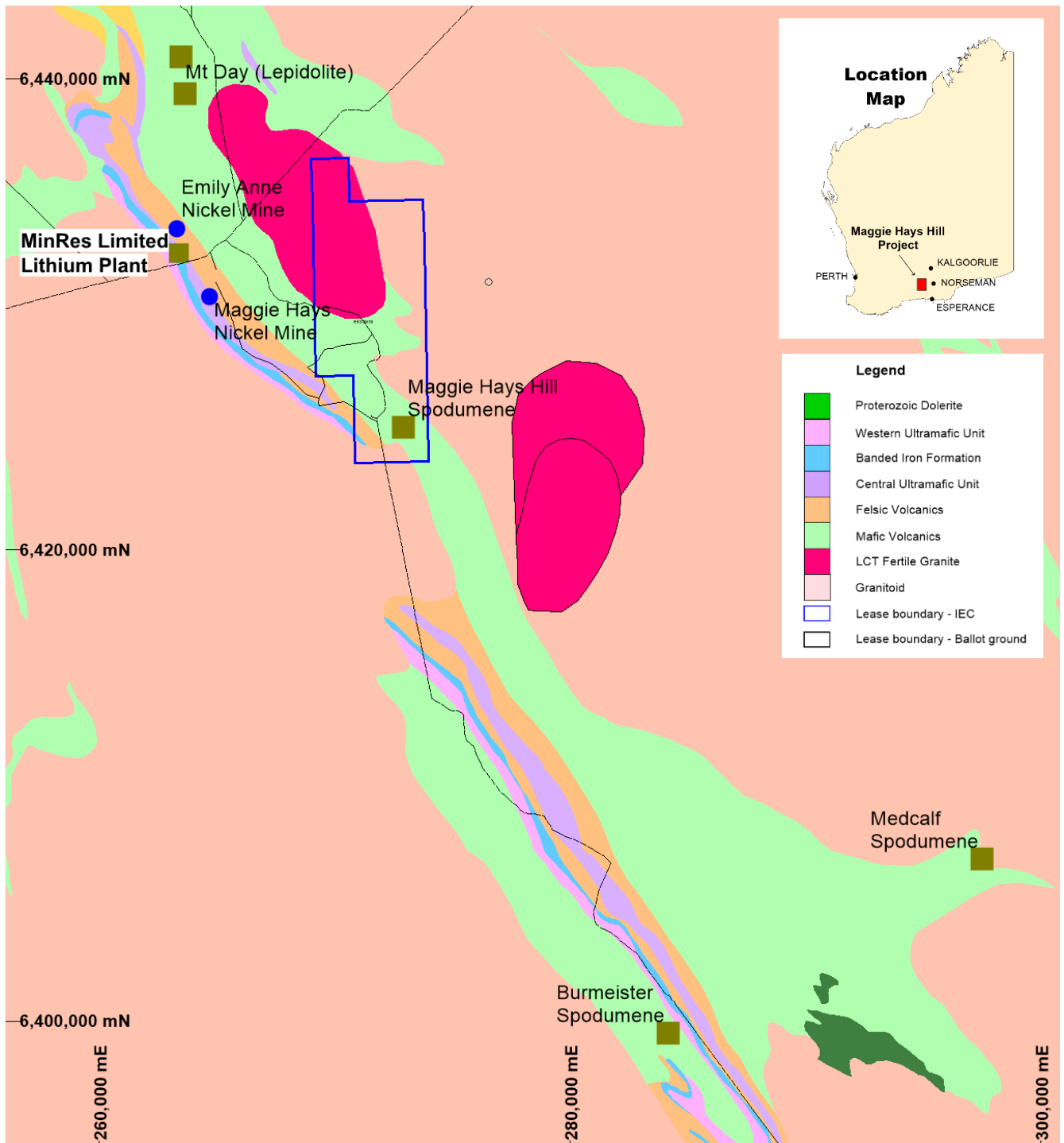
Figure 4. Tenement location map overlaid on geology showing regional lithium deposits.
