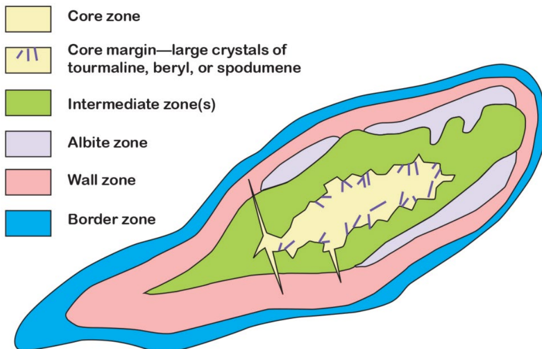
Figure 2. Deposit-scale zoning patterns in an idealized pegmatite (USGS 2016).
