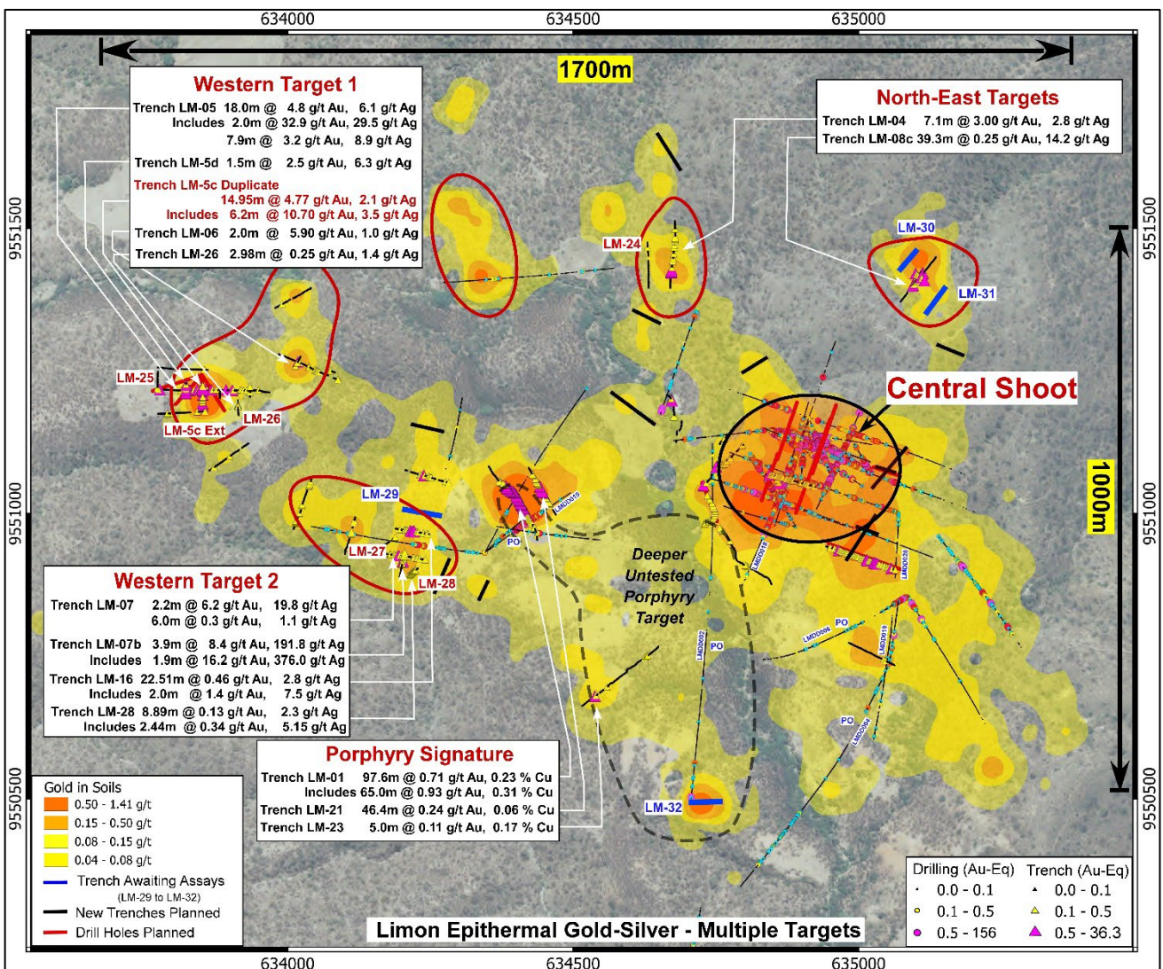
Figure 2: Limon gold-in-soils map showing extensive anomalous gold over an area of 1.7km x 1.0km. The circled areas have seen only partial testing and show epithermal gold-silver domains. Intersections in trenches LM-5c, and LM-19 to LM-23 from recently received assays are shown together with prior trench intersections. The black dashed line shows the Limon porphyry target outline.
