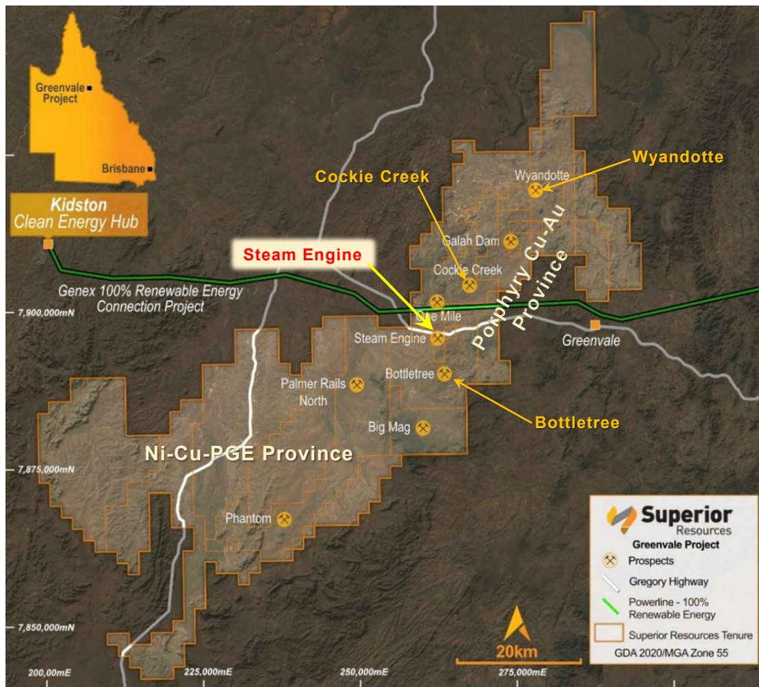
Figure 1. Map showing the location of the Steam Engine Gold Project within the Greenvale Project tenements and select prospects. The Gregory Highway and the Renewable Energy Power Infrastructure Corridor are also shown.
