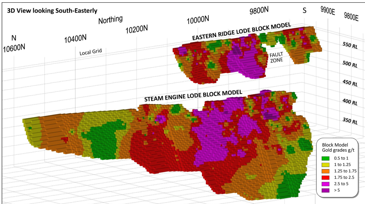
Figure 6. Oblique 3D view (from above GL) of the Steam Engine and Eastern Ridge lode block models (1.0g/t Au cut-off).
