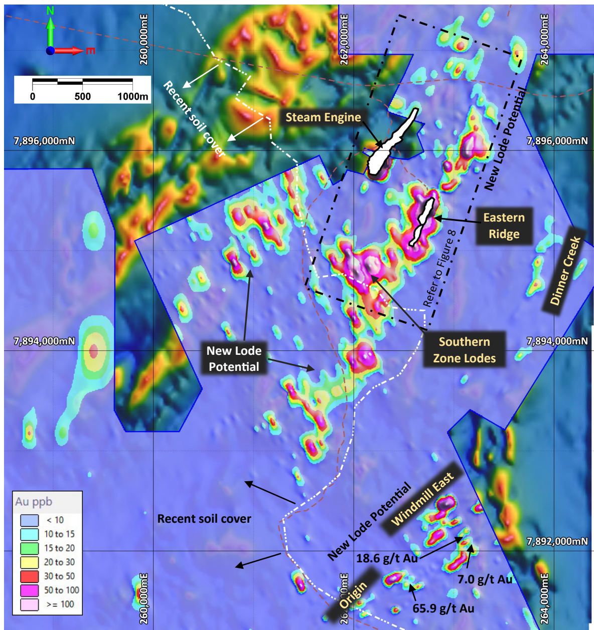
Figure 9. Plan showing gridded Au soil geochemistry over background RTP airborne magnetics data. The Steam Engine and Eastern Ridge lode Mineral Resource outlines are shown as white polygons together with areas of potential new lode zones. The Southern Zone, Windmill East and Origin mineralised zones are also shown.
