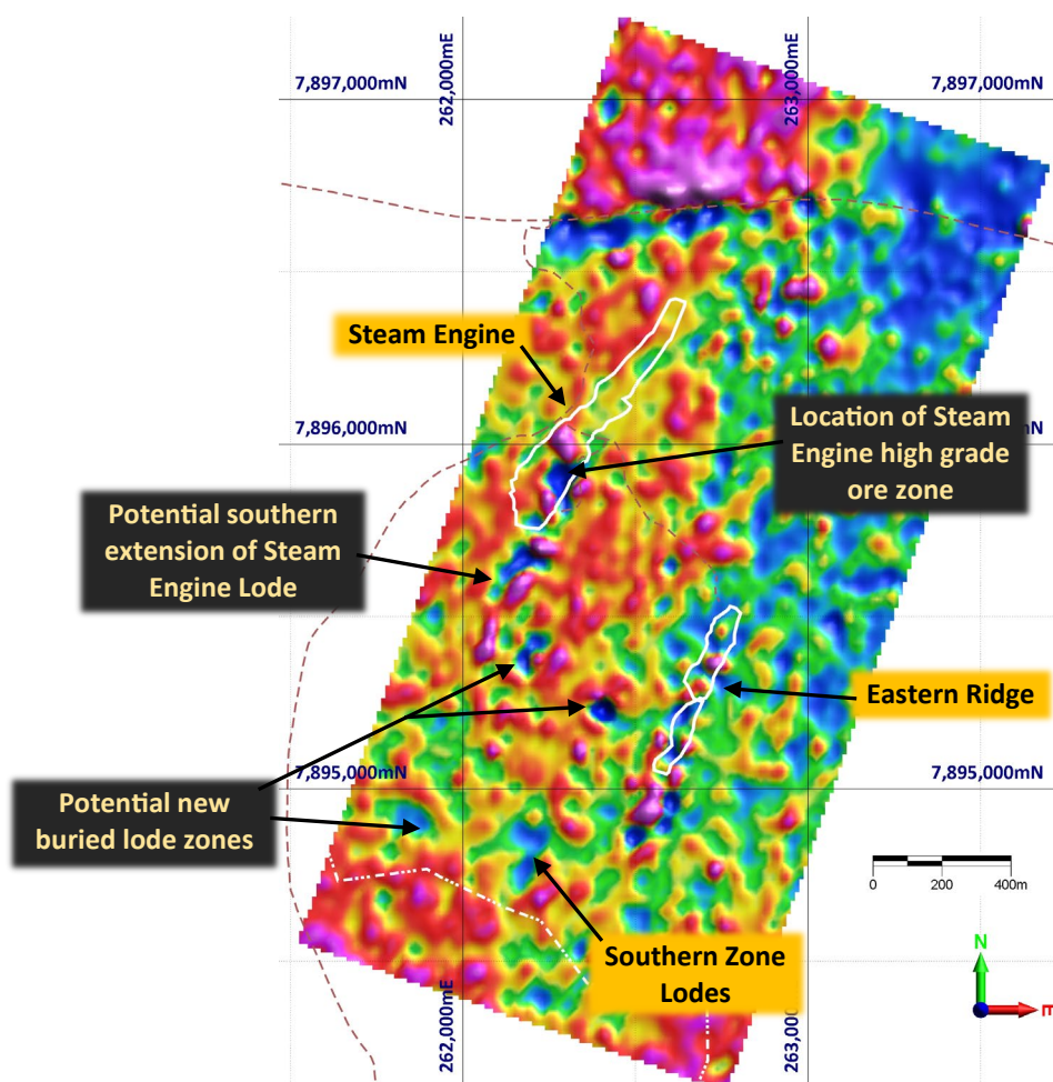
Figure 10. Image of late channel (Channel 16) total field electromagnetics (TFEM) responses over the Steam Engine and Eastern Ridge lodes. Discrete areas of low TFEM response are coincident with the most intensely mineralised parts of the gold lodes. A possible southern extension to the Steam Engine Lode is visible as well as other potential lode zones.
