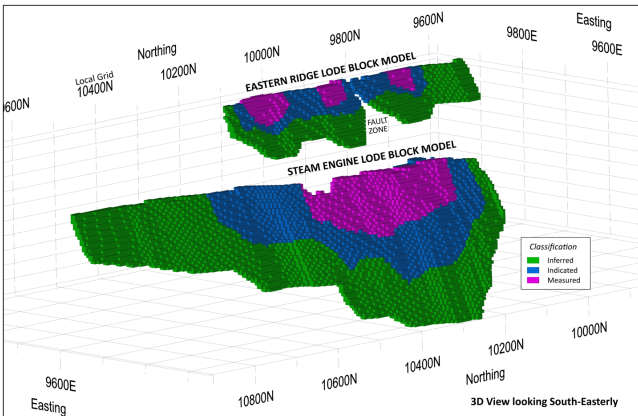
Figure 7. Oblique 3D view (from above GL) of the Steam Engine and Eastern Ridge lode high-grade block models (1.0 g/t Au cut-off) showing JORC, 2012 Measured, Indicated and Inferred confidence categories.
