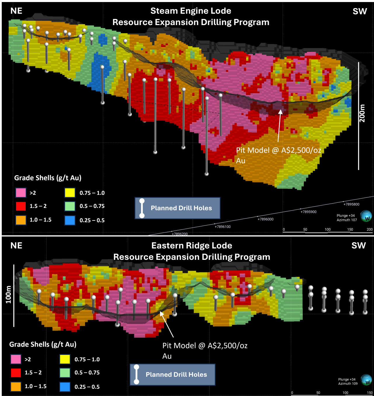
Figure 3. Block models of the Steam Engine and Eastern Ridge lodes showing the forward Resource expansion drilling program. Optimised pit shell models (@$2,500/oz Au) developed for the 2021 Scoping Study are also shown.
