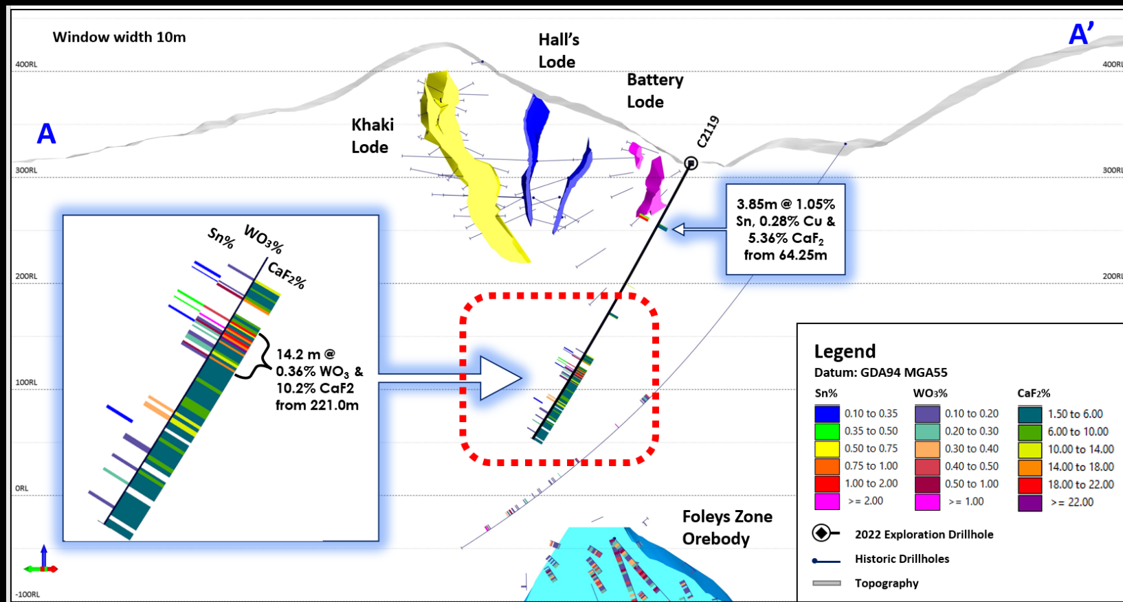
Section A-A' of C2119 Drilling (with assays plotted) looking northeast.
