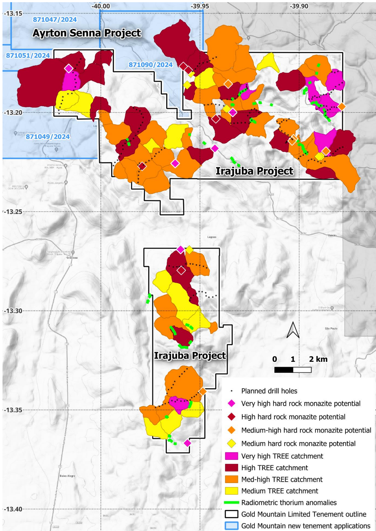
Figure 1. TREO anomalies plotted as anomalous stream sediment catchments. Maximum value of 4,582 ppm TREO. New data added additional very high TREO values in the highest (purple) category.
