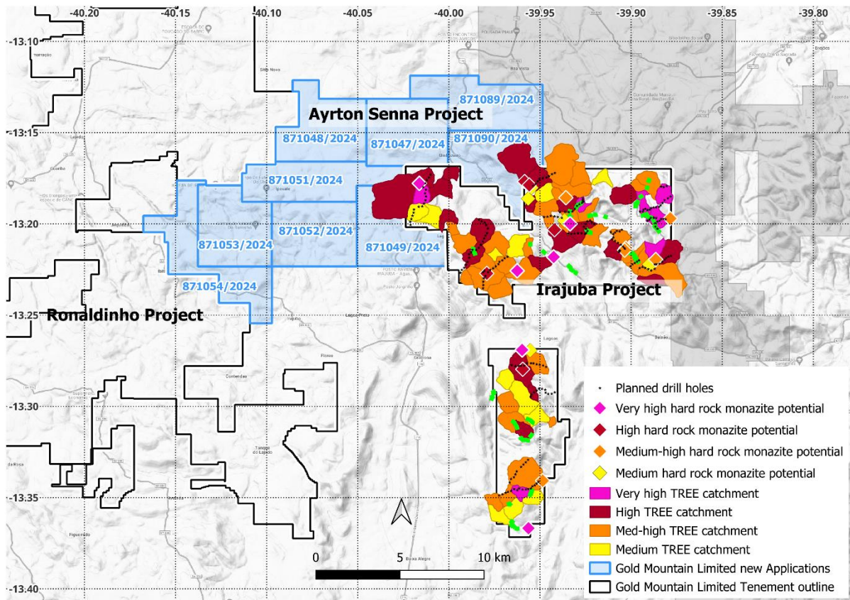
Figure 4. New tenement applications lodged and accepted by the ANM covering part of the anomalous catchments from Irajuba.
