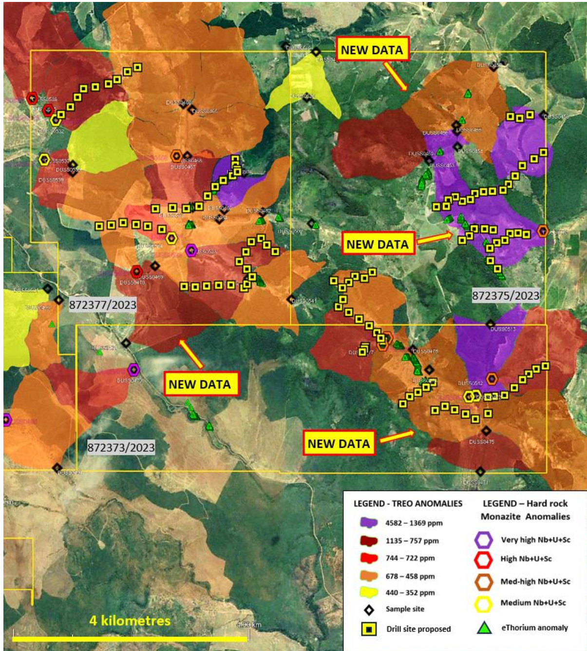
Figure 2. Detail of the northeastern part of the Irajuba tenements showing anomalous areas consolidated and extended with the new results. Additional drill hole traverses have been designed for approval to cover the new areas.
