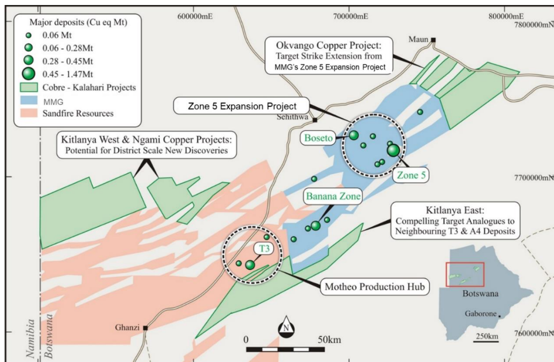
Figure 8. Locality map illustrating the position of the Cobre license holding in the KCB relative to known deposits and production hubs.
