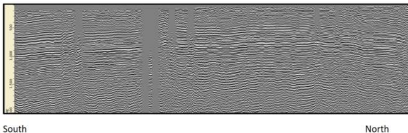
Figure 5: uninterpreted Blue processed Line 23GA NT1-B showing continuous (presumed) Proterozoic aged sedimentary reflectors down to 1.2 seconds TWT from the north to south through EP 205 and 207 and Blue's application area EP 211. Source: Blue Energy.
