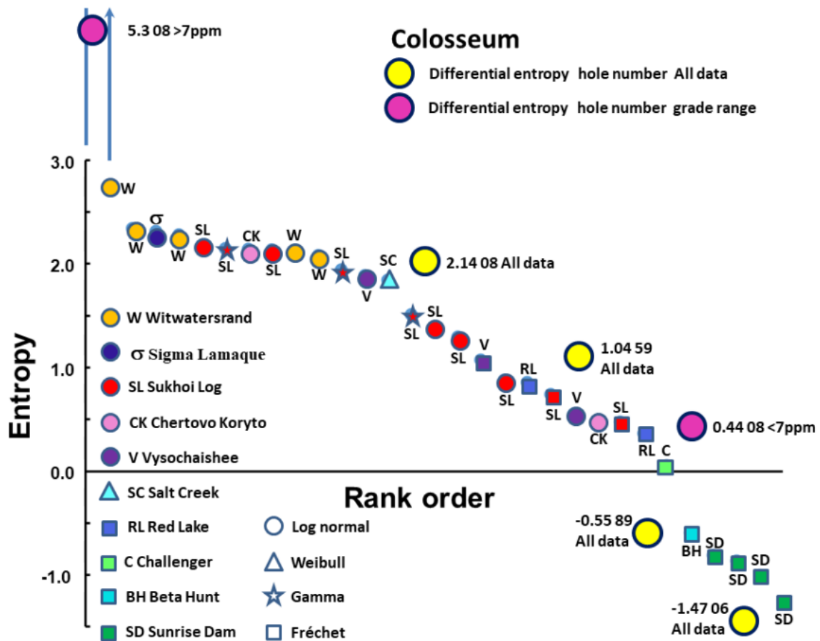
Colosseum data for holes 06, 89, 59 and 08 superimposed on Figure 5 of Ord and Hobbs (2023, https://doi.org/10.1080/08120099.2023.2207628 ). Differential entropy for individual drill holes from gold deposits of various quality in rank order. Each colour represents a geographical location for the data. Each symbol represents the best-fit probability distribution function for those data. Note that the data for hole 08 separated clearly into greater than and less than 7 ppm groups.
