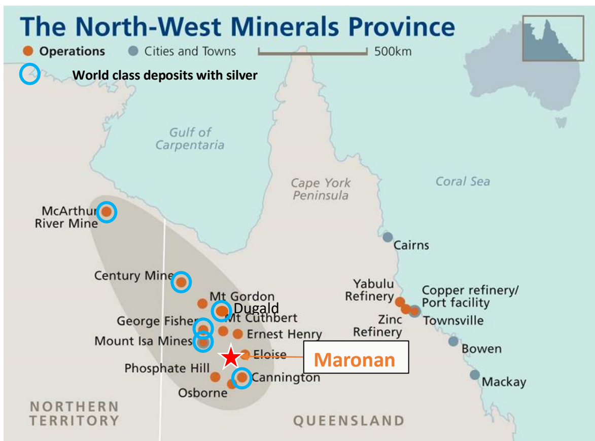
[Figure 1] Northwest Minerals Province – Maronan Location
