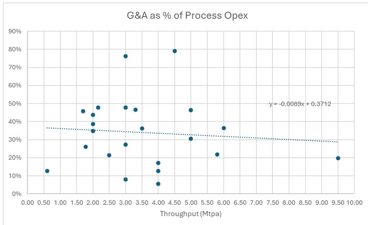
Figure 26: Benchmarking of General and Administration Costs
