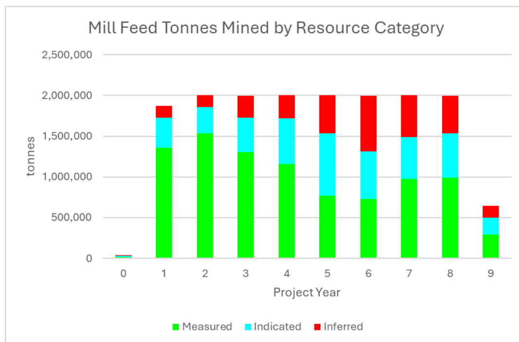
Figure 17: Tonnes Mined by Resource Category
