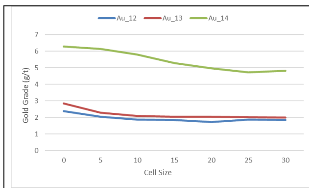
Figure 4-6. Cluster analysis – gold domains
