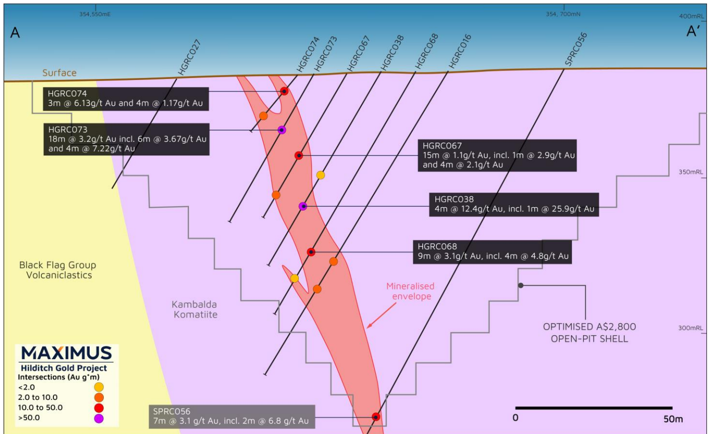
Figure 3 – Hilditch gold deposit– North-looking cross-section at 6536370mN (±5m), illustrating mineralised envelope, gold assay intersections, and optimised A$2,800 open-pit shell.
