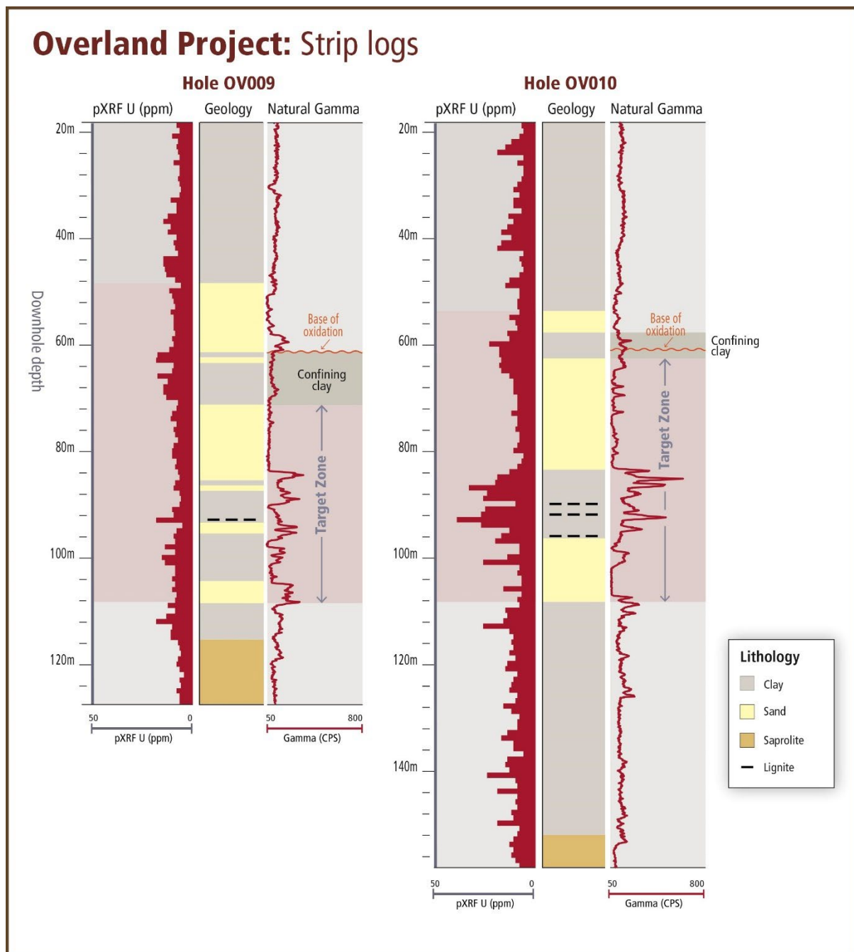
Figure 5: Downhole pXRF and natural gamma logs over target intervals for holes OV009 and OV010. In relation to the disclosure of pXRF results, the Company cautions that estimates of uranium elemental abundance from pXRF results should not be considered a proxy for quantitative analysis of a laboratory assay result. Assay results are required to determine the actual widths and grade of the mineralisation.
