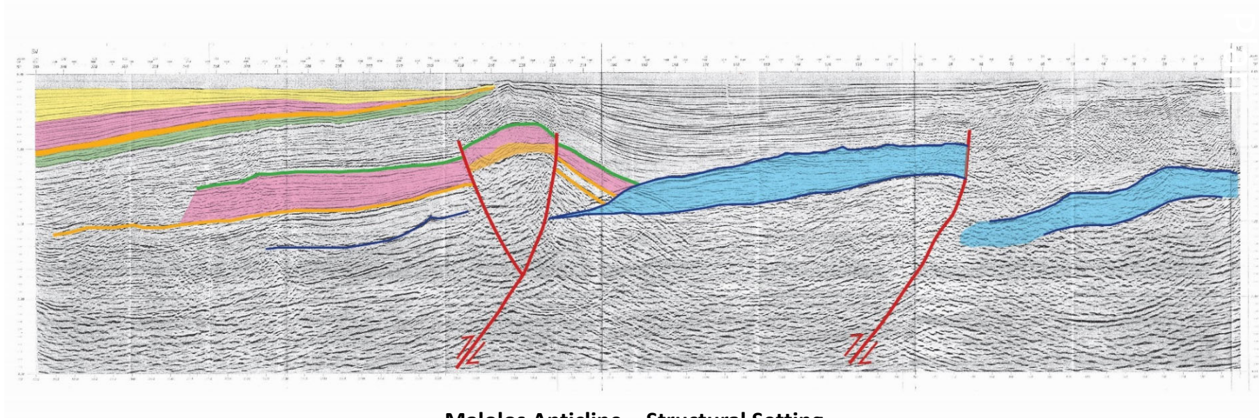
Malolos Anticline – Structural Setting
