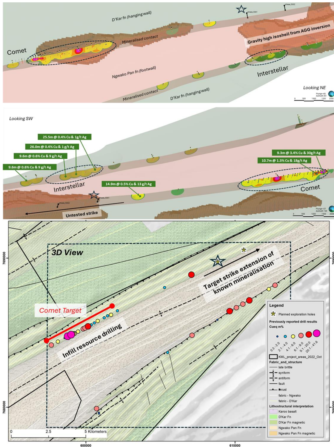
Figure 1. 3D view (top two panels) from the SW and NE and plan view illustrating target areas for exploration drilling and infill resource drilling on interpreted and modelled lithology. Drill hole NCP55 is highlighted with a star. Notable intersections and dense portions of the AGG inversion highlighted.
