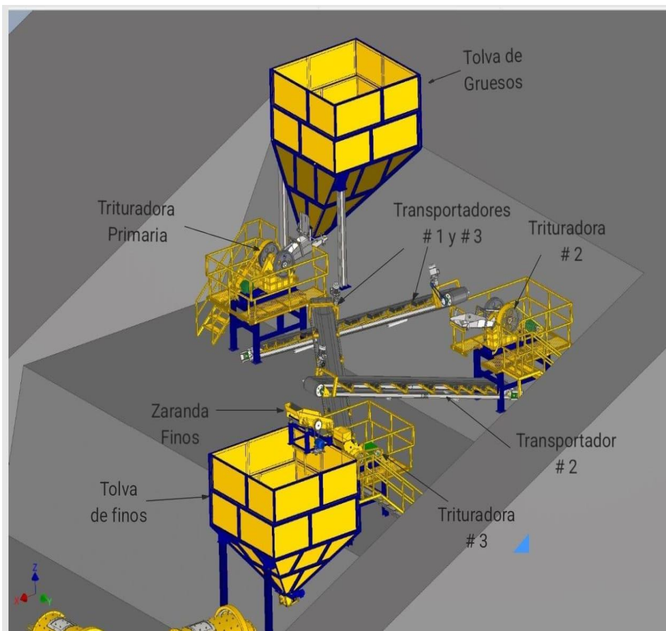
Photo 3 : NEW 3 STAGE CRUSHING CIRCUIT DESIGN
