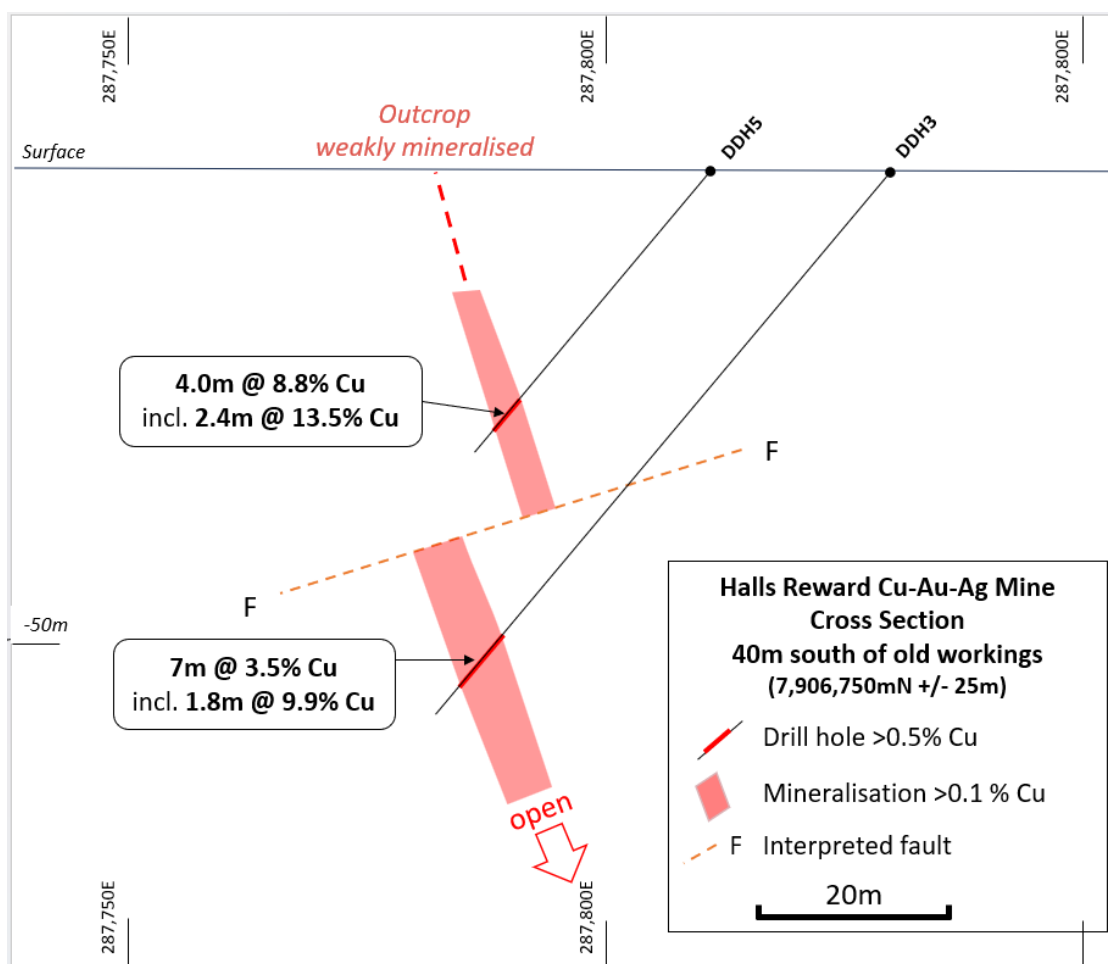
Figure 3. Cross section showing high-grade drilling intersections 35m south of historically stope areas.
