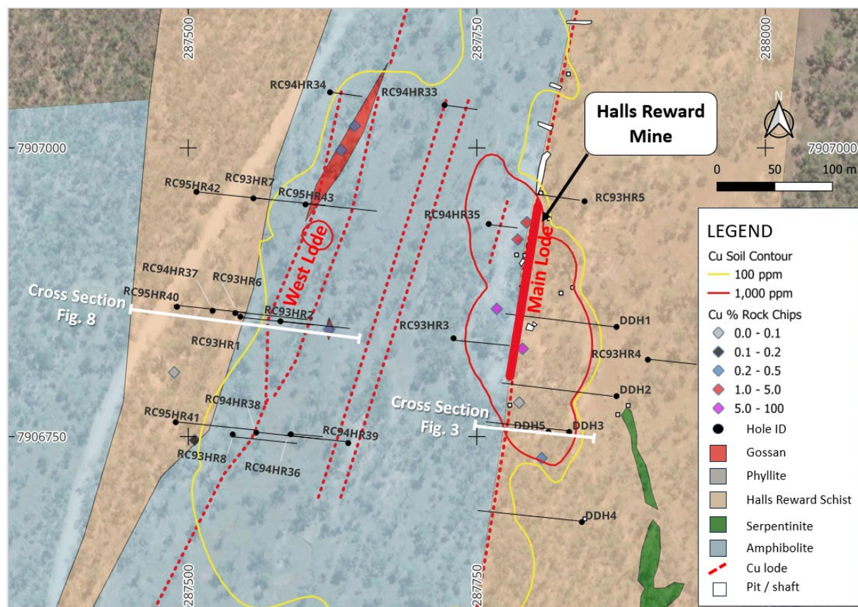
Figure 5. Drill collar plan showing diamond core holes targeting the Main Lode and CRAE's RC holes mainly targeting the West Lode gossan and geochemical anomaly.
