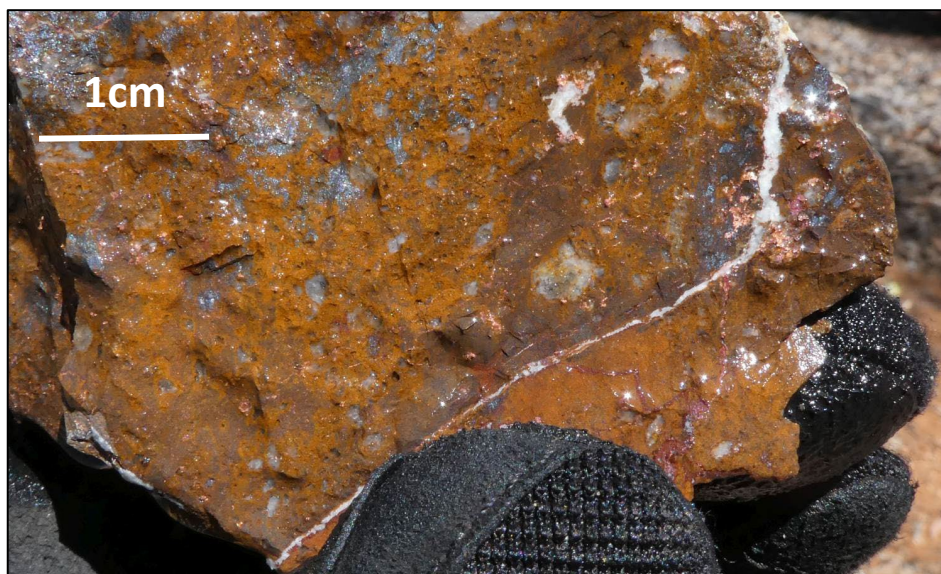
Figure 6. Main Lode silicious gossan grading 20.13 % Cu, 0.21 g/t Au, 58 g/t Ag with native Cu on fractures (pink metallic lustre) and chalcocite (grey).
