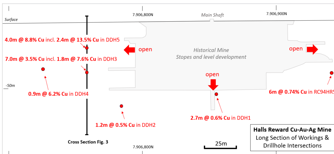
Figure 2. Long section view of Halls Reward mine looking west, showing stoped areas to 50m below surface, and historical drilling intersections. Mineralisation is open in all directions; exceptional high-grade material remains in situ to the south.
