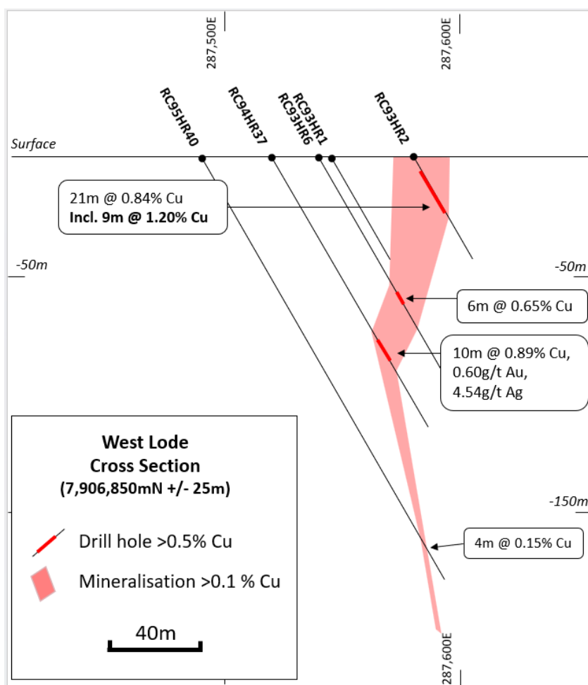
Figure 8. Cross section through West Lode, showing significant mineralisation at shallow depths.
