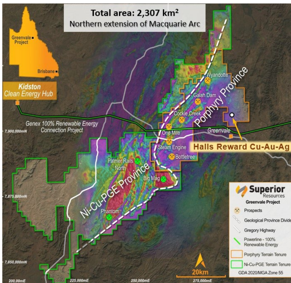
Figure 1. Greenvale Project regional magnetics with the location of the high-grade Halls Reward Cu-Au-Ag mine. Additional nearby high-grade Cu deposits include Wyandotte and One Mile, alongside the Company's large-scale porphyry Cu-Au discoveries at Bottle Tree and Cockie Creek.
