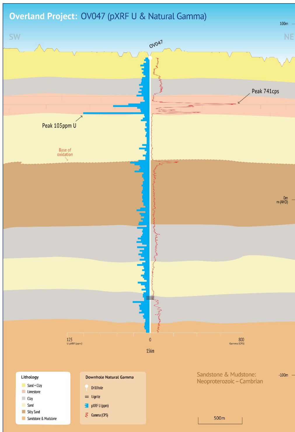
Figure 1: Strip log displaying drillhole OV047 lithology, natural gamma responses (cps) and pXRF uranium responses (ppm U). In relation to the disclosure of pXRF results, the Company cautions that estimates of uranium elemental abundance from pXRF results should not be considered a proxy for quantitative analysis of a laboratory assay result. Assay results are required to determine the actual widths and grade of the mineralisation. The company uses an Olympus Vanta M Series portable X-ray Fluorescence (pXRF) analyzer to screen Air Core drilling samples for mineralization prior to submitting samples to a commercial laboratory for assay. This provides an initial understanding of the mineralization distribution before sampling, ensuring submitted samples are representative of the targeted mineralization. While pXRF confirms the presence of mineralization, it does not accurately determine elemental concentrations due to limitations such as a small analysis window, uneven distribution, shallow penetration depth, and irregular surfaces. The pXRF results are indicative and the pXRF readings are subject to confirmation by chemical analysis from an independent laboratory.
