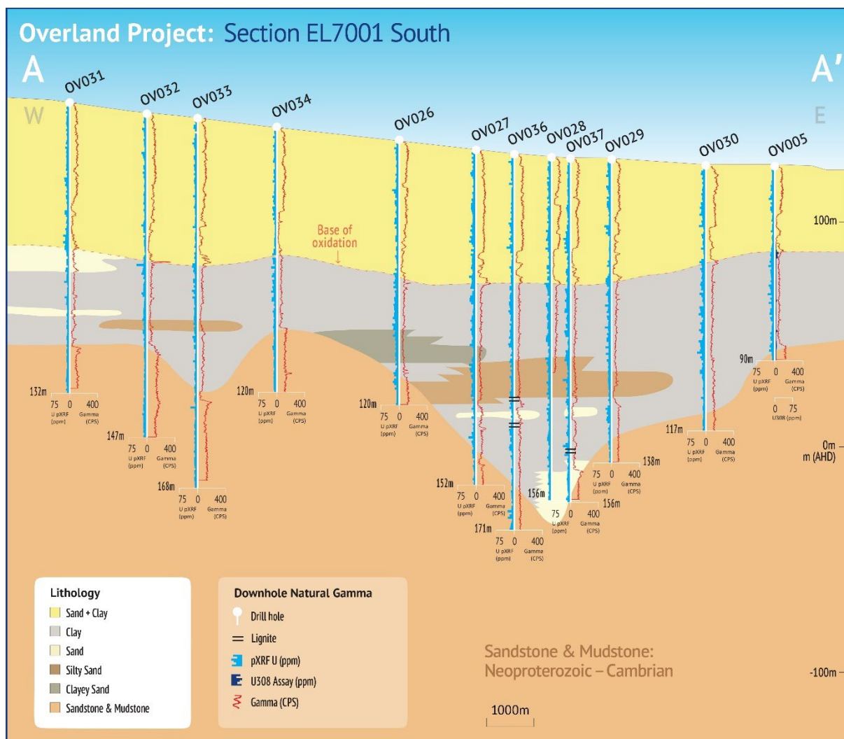
Figure 3: Cross section A-A' across the defined palaeovalley showing lithology, pXRF U (ppm), and Gamma (CPS) see Figure 2 for section location plan.
