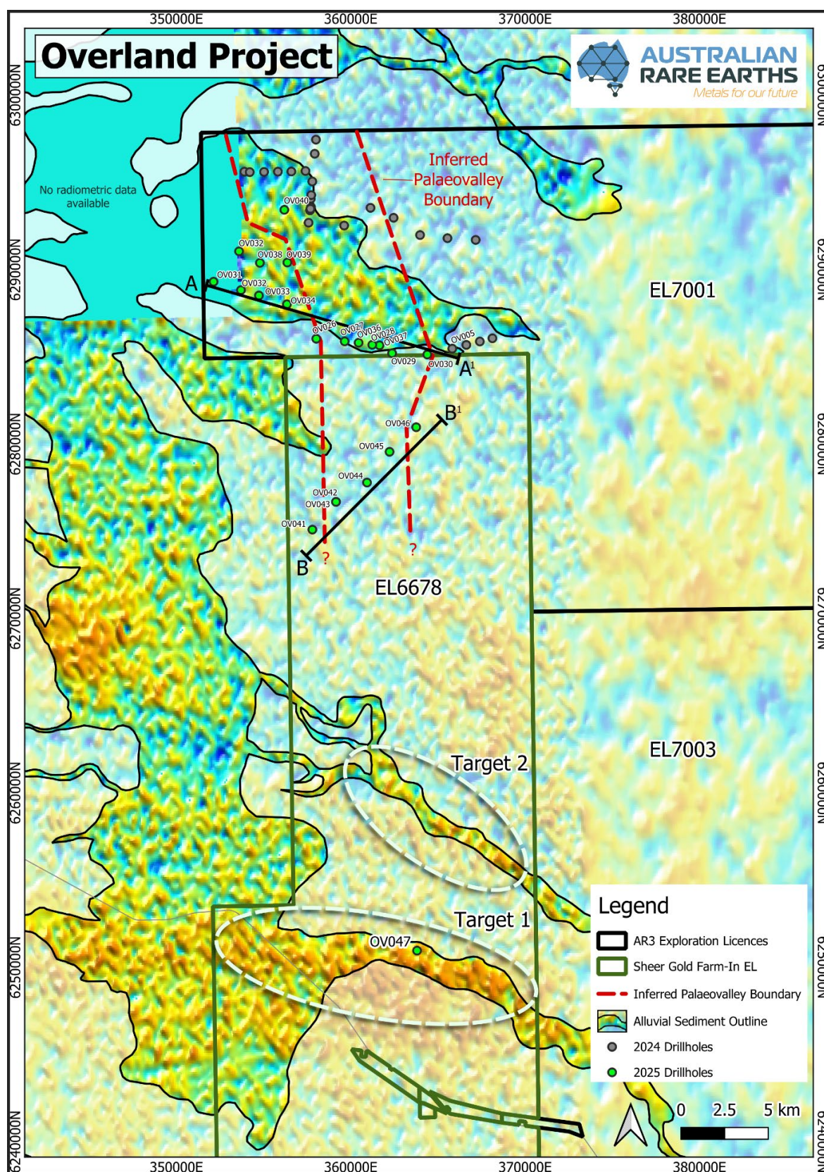
Figure 2: Overland drilling (2024 & 2025) with airborne radiometrics, alluvial sediment channels, and interpreted palaeochannel boundary based on recent drilling. Target 1/OV047 has been prioritized for follow up drilling. Note: The airborne radiometric image and Alluvial Sediment Outline is publicly available data sourced from SARIG ( https://map.sarig.sa.gov.au ) and detailed within the appendices of this report.
