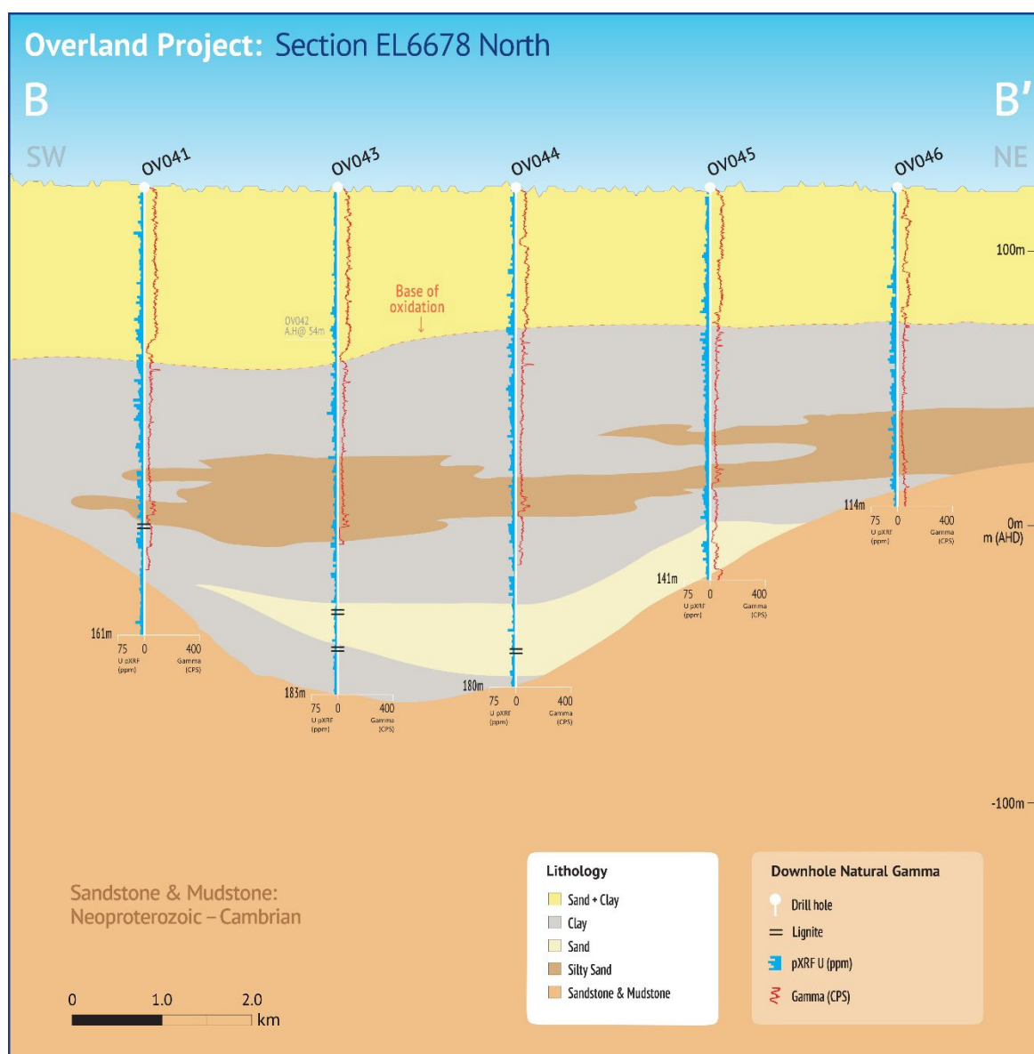
Figure 4: Cross section B-B' across the defined palaeovalley showing lithology, pXRF U (ppm), and Gamma (CPS) see Figure 2 for section location plan.
