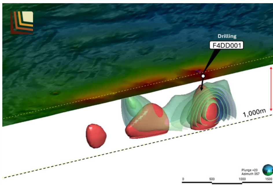
Figure 3. F4 anomaly 3D magnetic inversion model anomaly shells (Red >0.006 SI) and gravity anomaly modelled density shells (green >2.72 ) with surface showing magnetic RTP (section 6613500mN, MGA94 z54).
