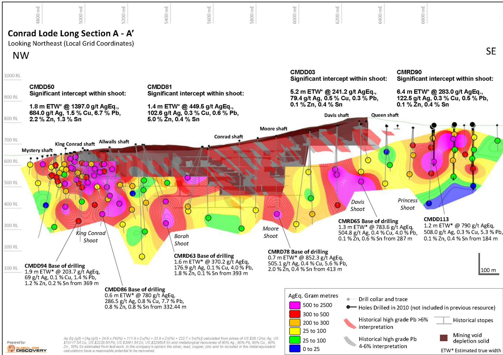
Figure 5: Conrad Silver Project Long Section
