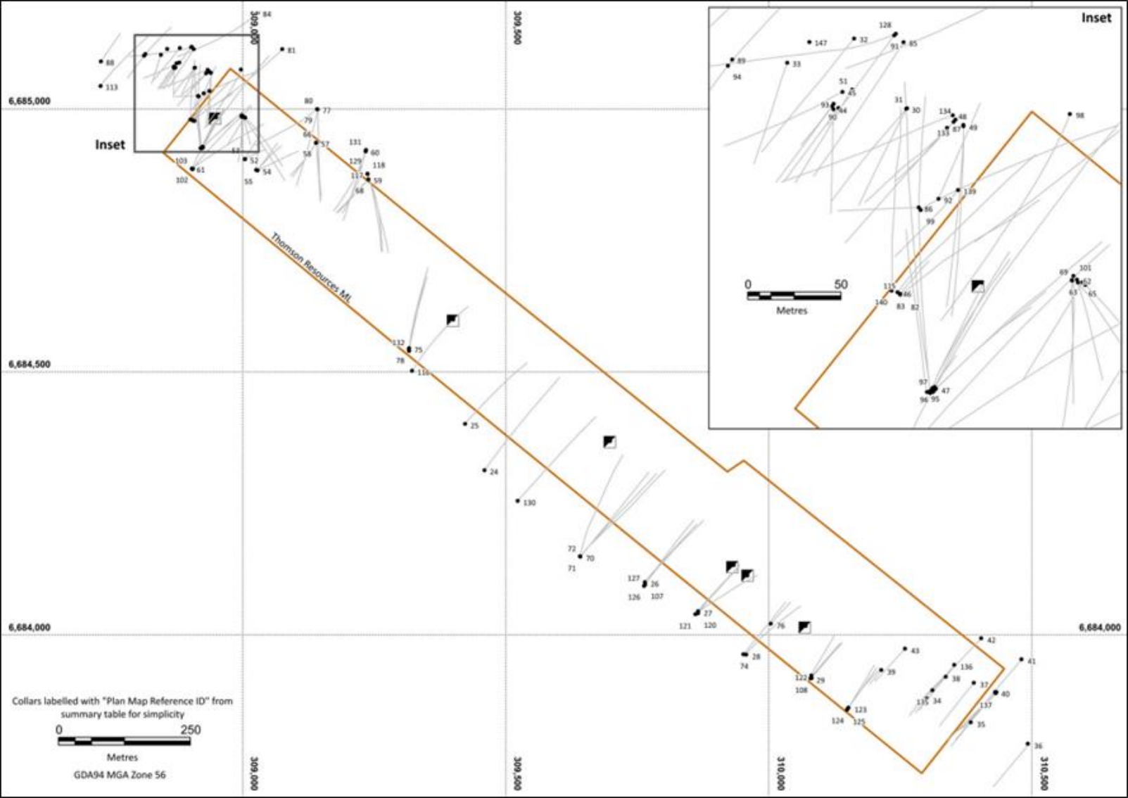
Figure 4: Conrad Silver Project Plan view
