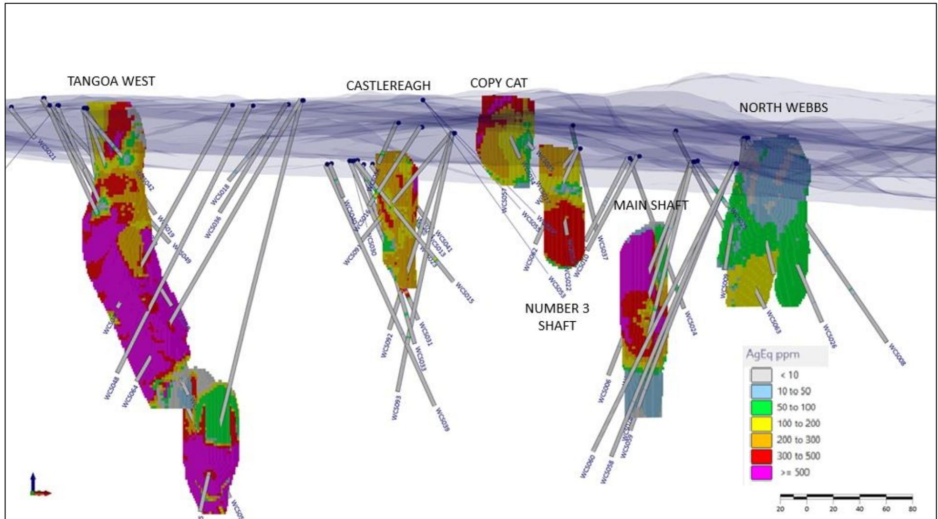
Figure 3. Long section of Webb's Consols mineralised pipes
