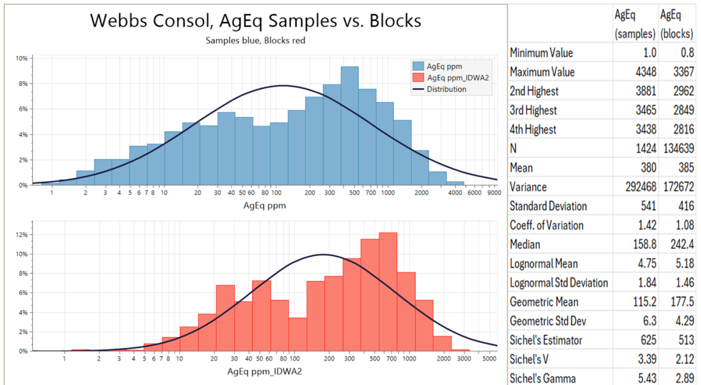
Figure 6. Histogram of 1m composite input data verses estimated block grades
