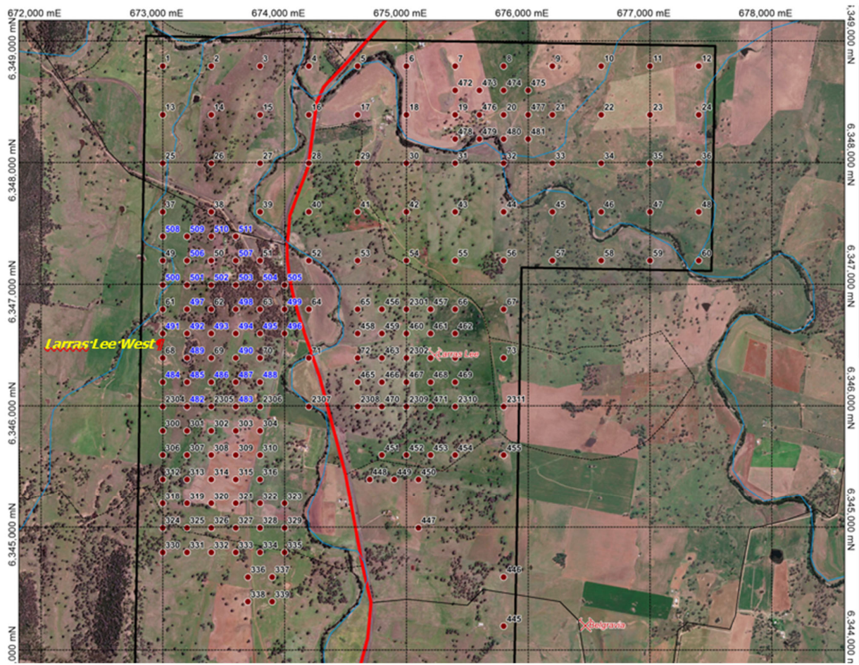
Figure 6: Geochemistry: Planned Infill Sampling – Larras Lee West
