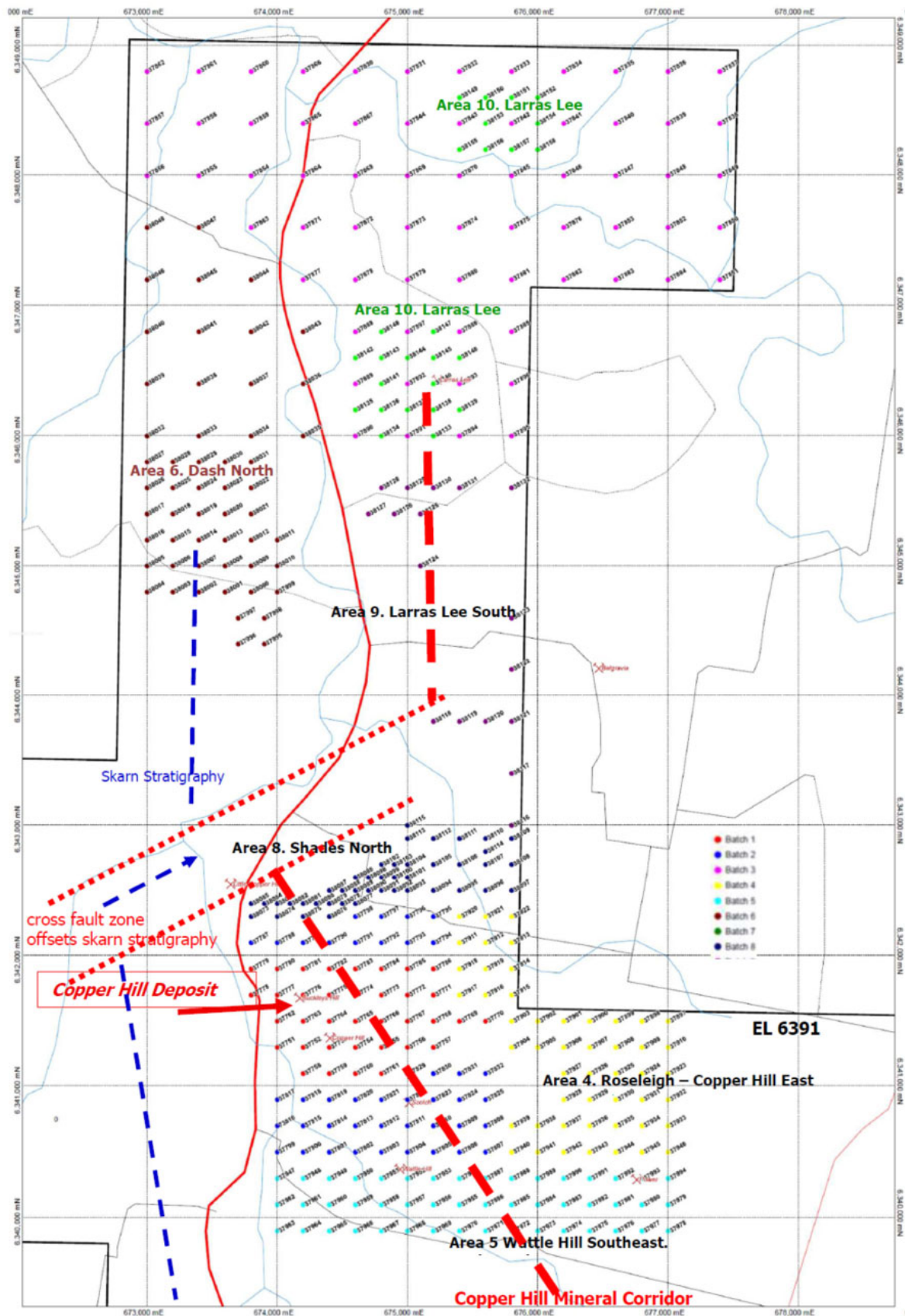
Figure 4: Geochemical Sampling sites – MGA Grid Northern EL6391
