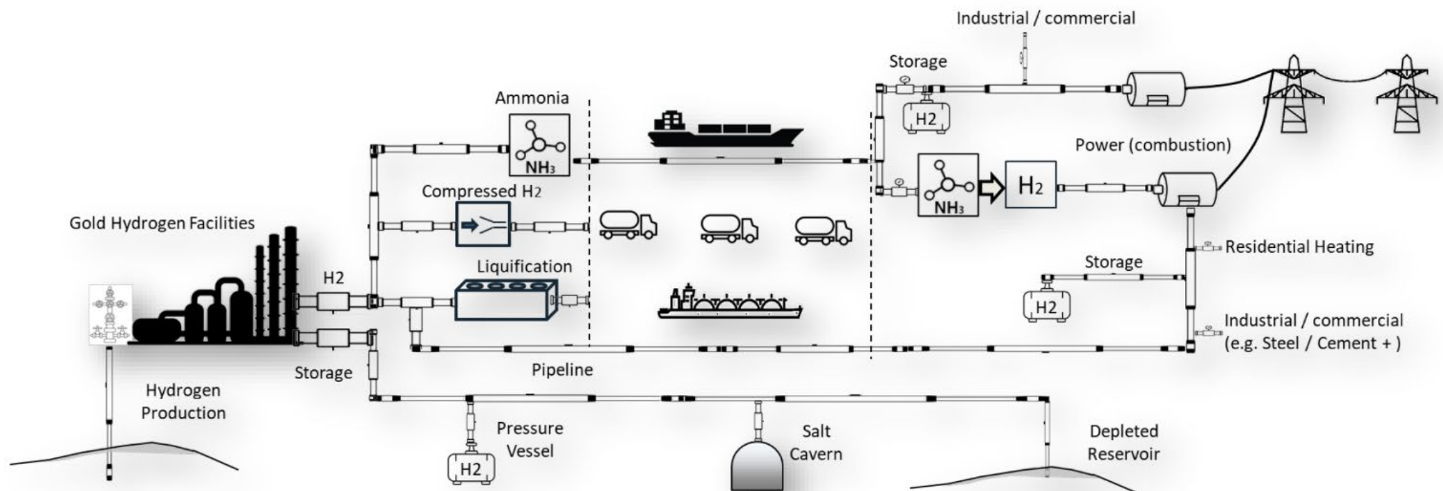
Figure 3 - Examples of downstream hydrogen distribution and usage
