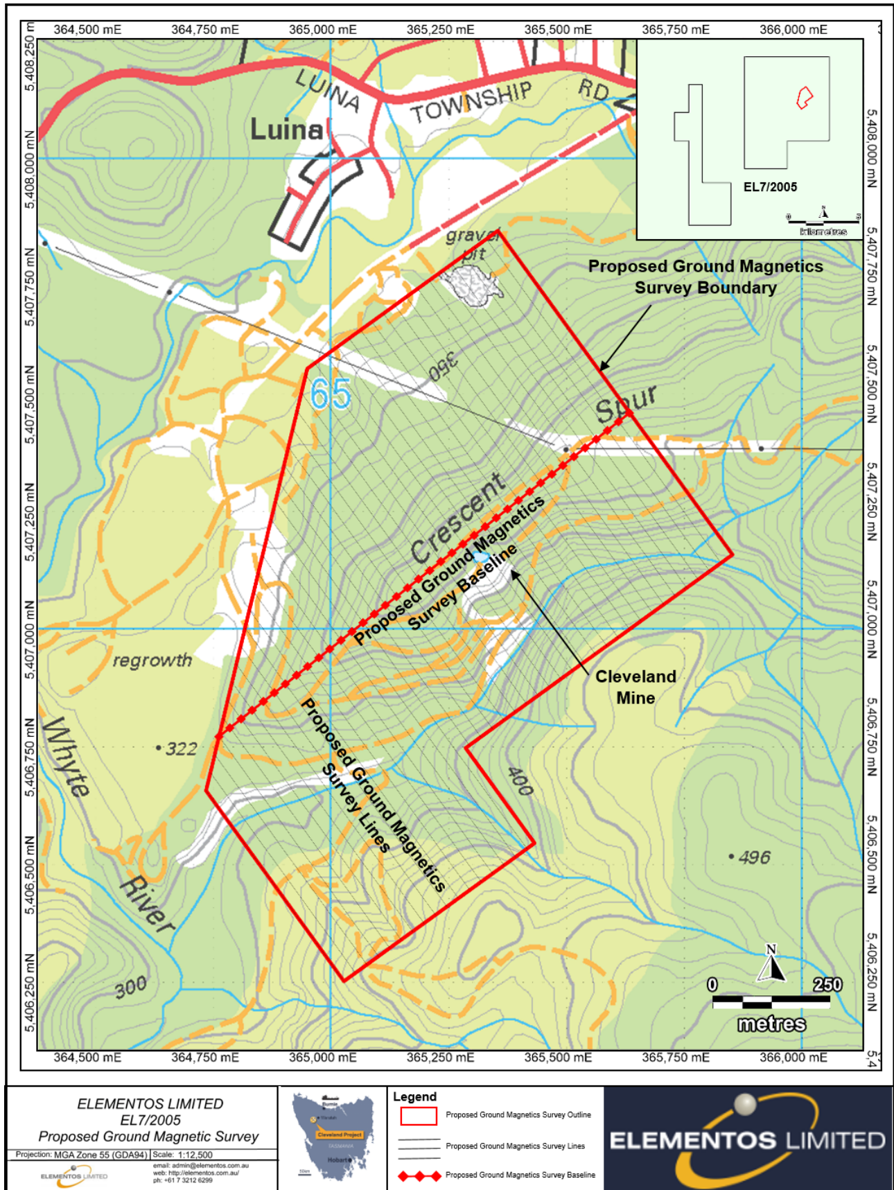
Figure 1: Proposed Ground Magnetic Survey
