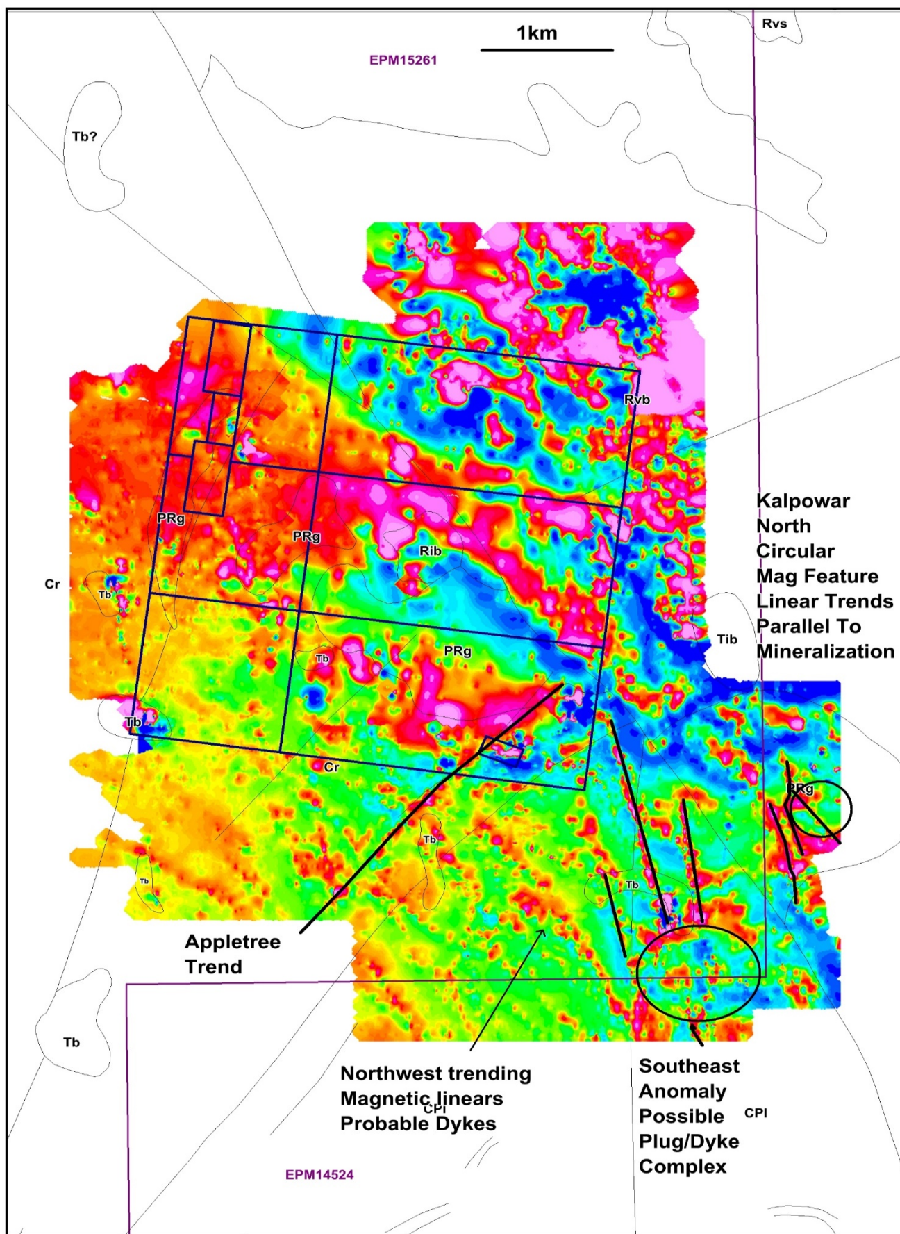
Figure 6: Ground Mag Survey Results 2015
