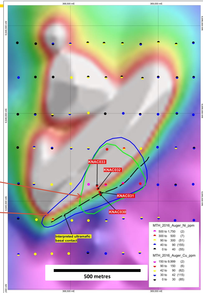
Magnetic image showing ultramafic basal contact, Ni - Cu surface anomaly and drillholes
