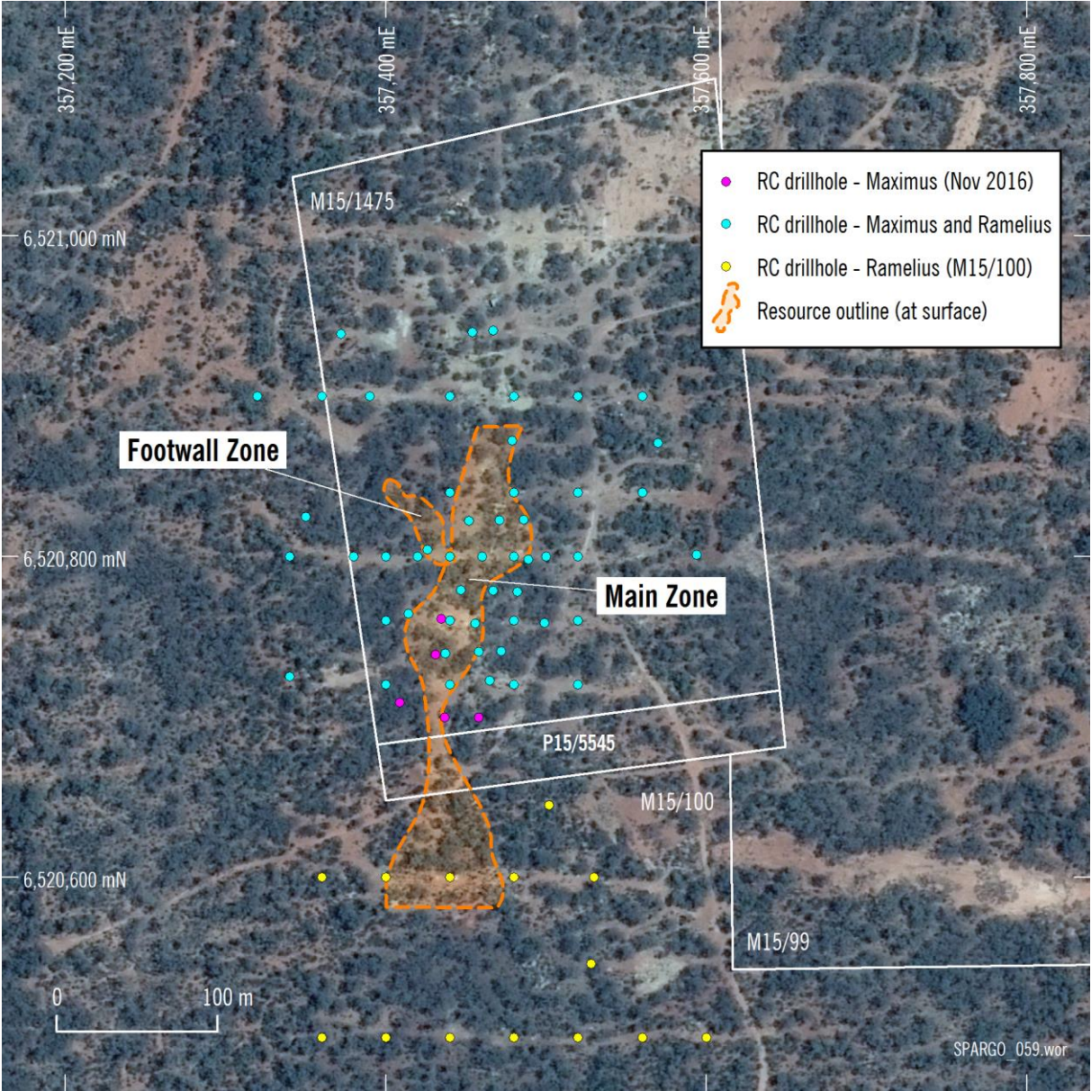
Figure 1: Map displaying the location of all drillholes used in the Mineral Resource estimate, and the location of the newly acquired tenement (P15/5545) to secure the southern extension of the ore body.
