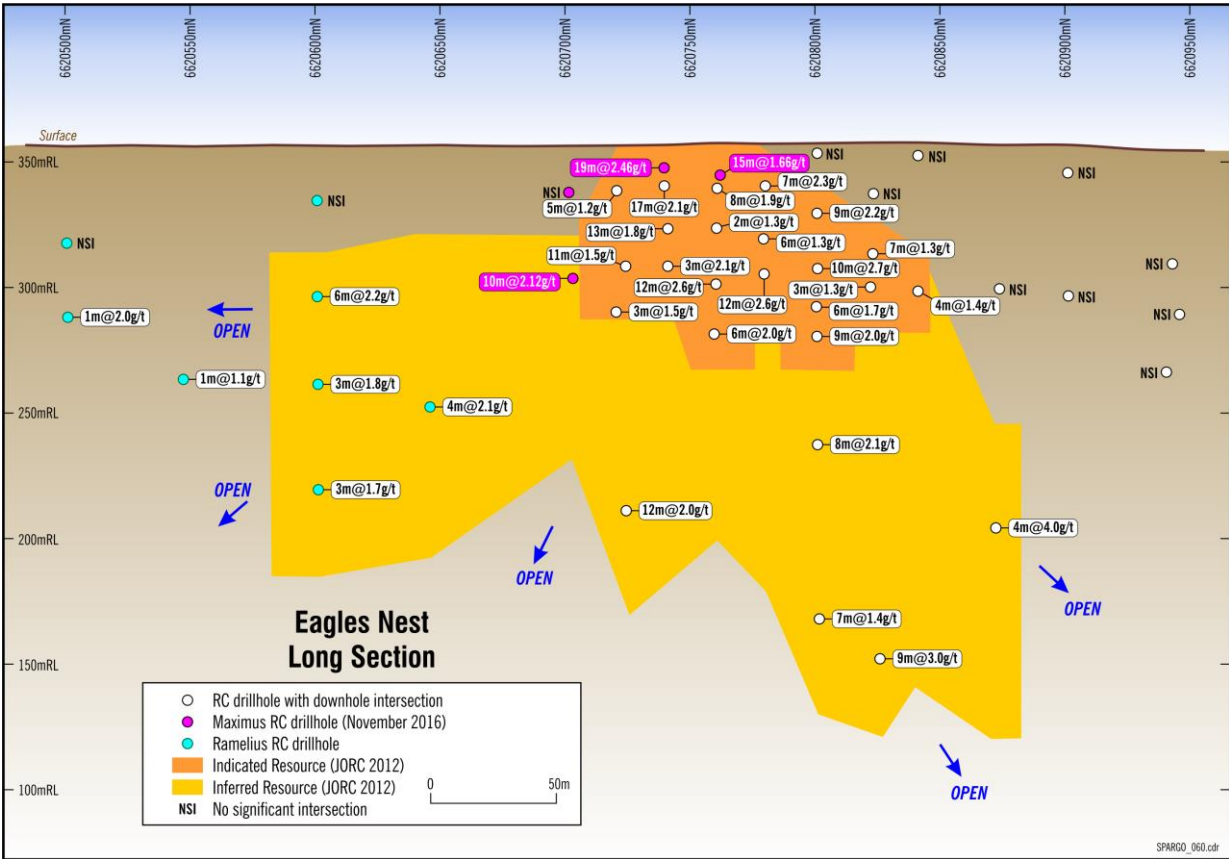
Figure 2: Eagles Nest long section – showing Mineral Resource estimate by classification
