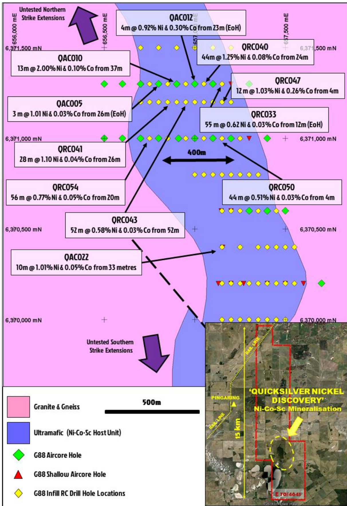
Figure 4 – Aircore & RC drill hole locations with significant nickel & cobalt intercepts over interpreted geology.
