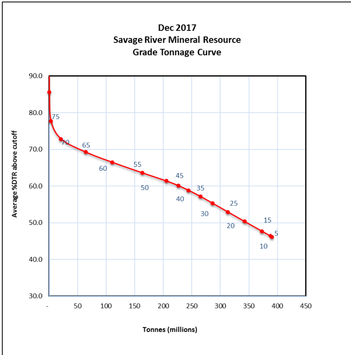
Figure 5 - Grade Tonnage Curve, Savage River
