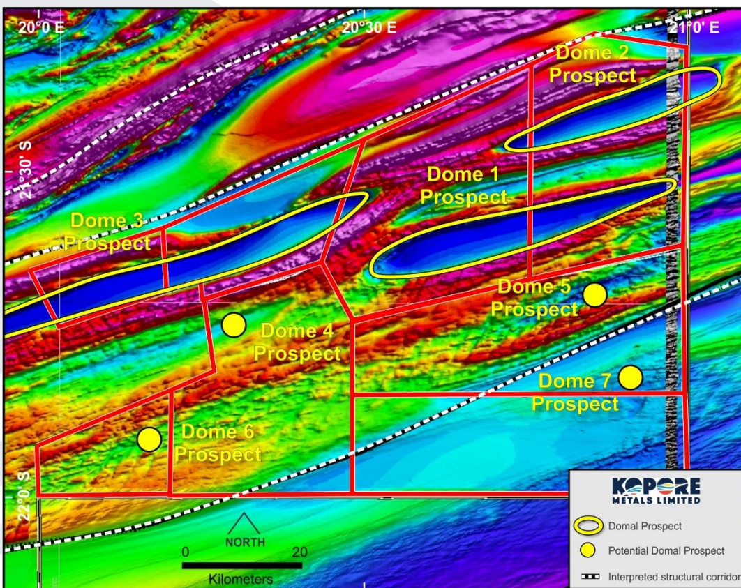
Figure 2 - Namibian Licences with geophysics showing interpreted domes and structural corridors
