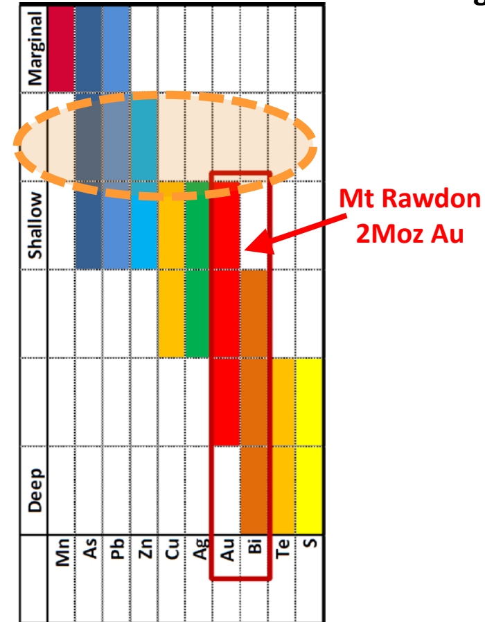
Mt Rawdon Gold Mine - Metal zoning
