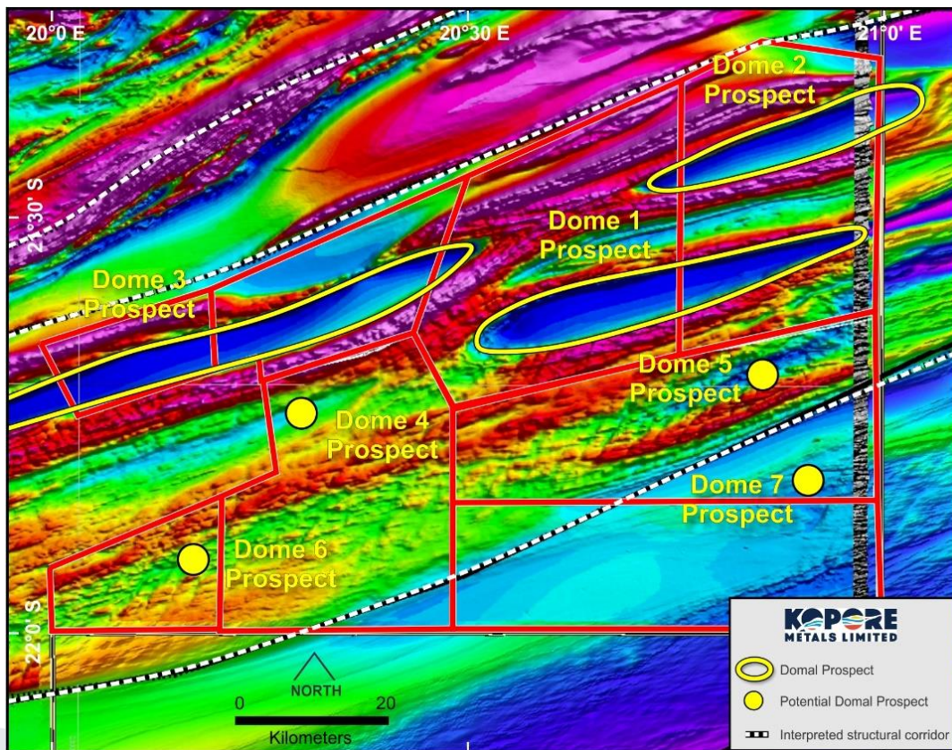
Figure 3. Interpreted domal prospects covering Namibian Licences 2
