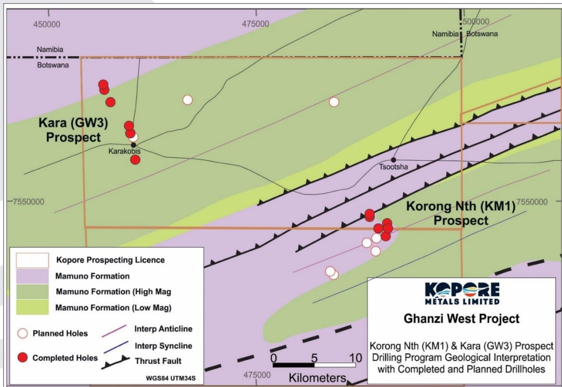
Figure 2 - Ghanzi West Regional Geology at the Korong Nth (KM1) and Kara (GW3) Prospects with Completed and Planned Drilling
