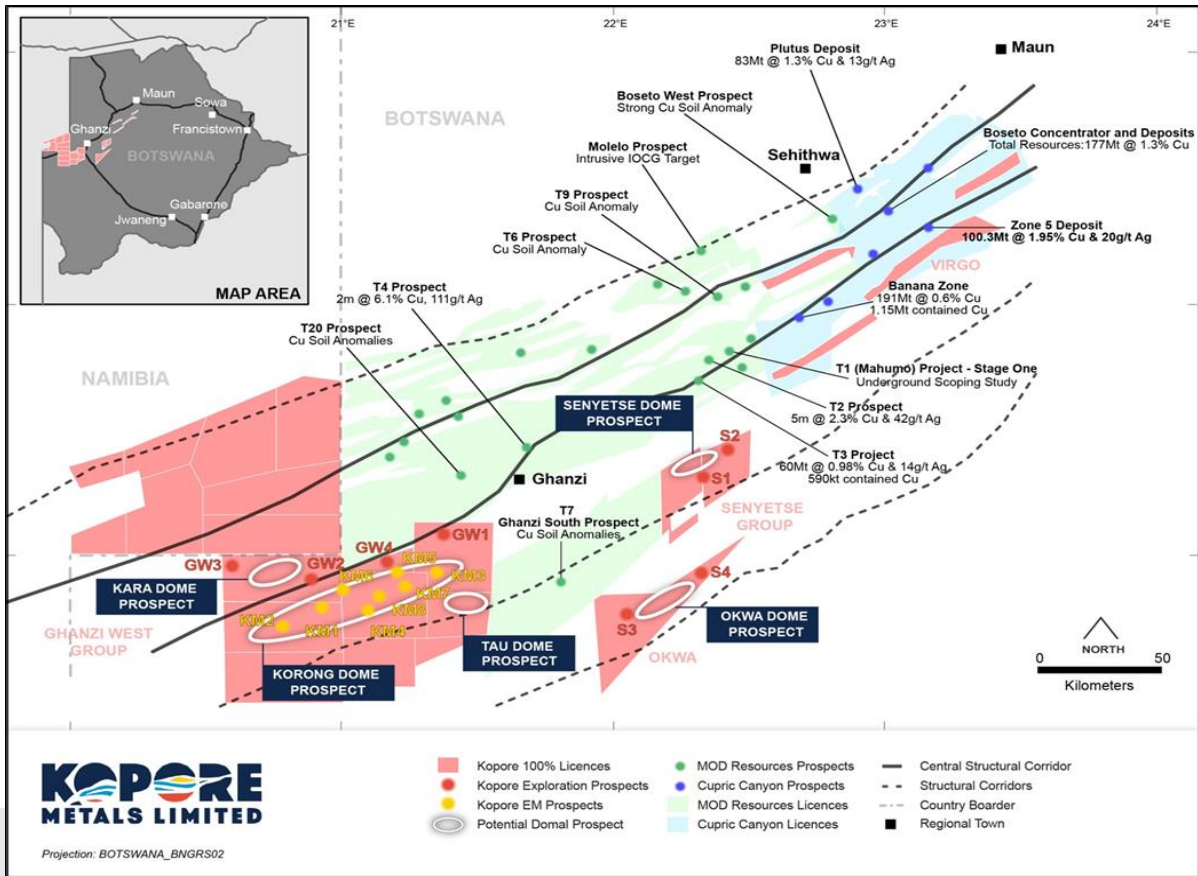
Figure 1 - Kopore Metals Prospecting Portfolio and Kalahari Copper Belt Regional Map
