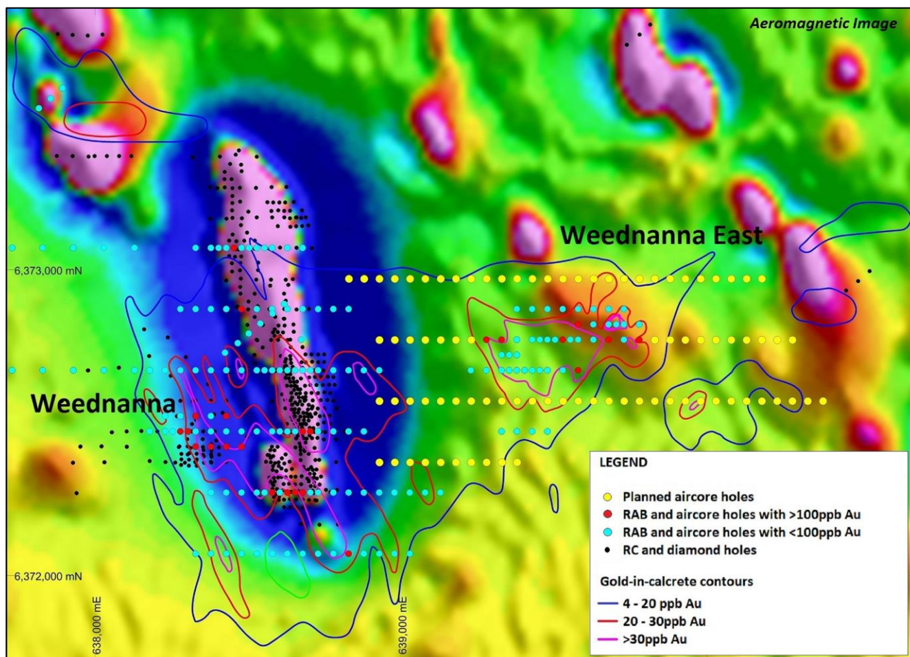
Figure 1. Weednanna East Prospect - Planned aircore holes with gold in calcrete contours
