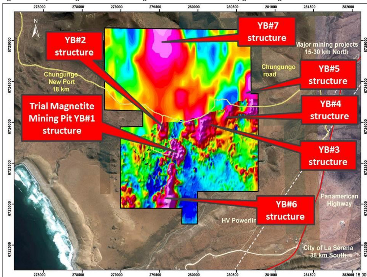
Figure 3 – Map showing the seven main magnetic structures identified by ground magnetics
