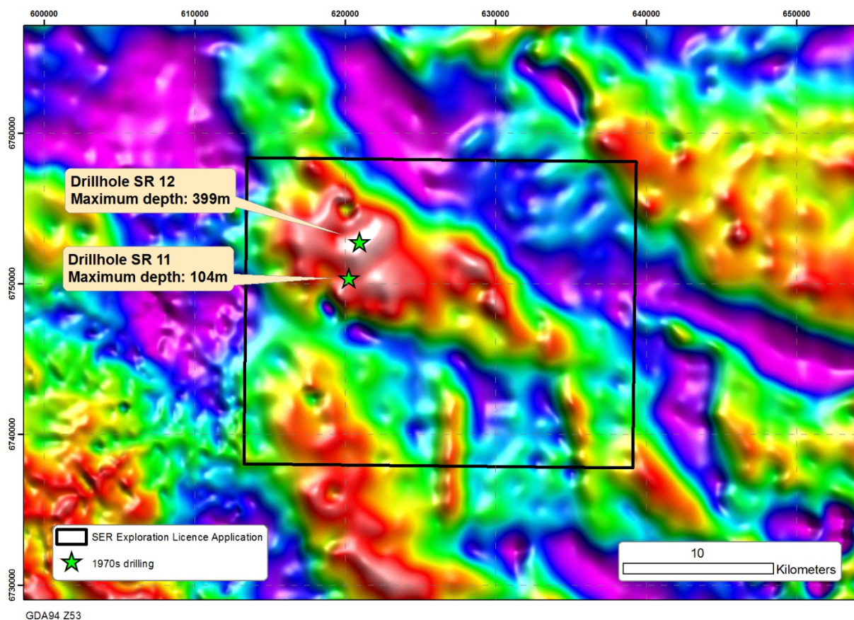
Figure 2: ELA 2018/185 Residual Bouguer Gravity Image
