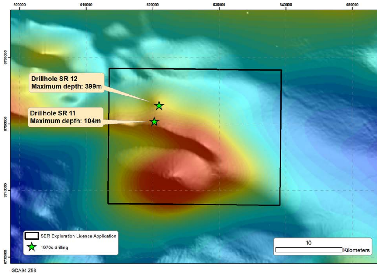
Figure 3: ELA 2018/185 RTP Magnetics Image
