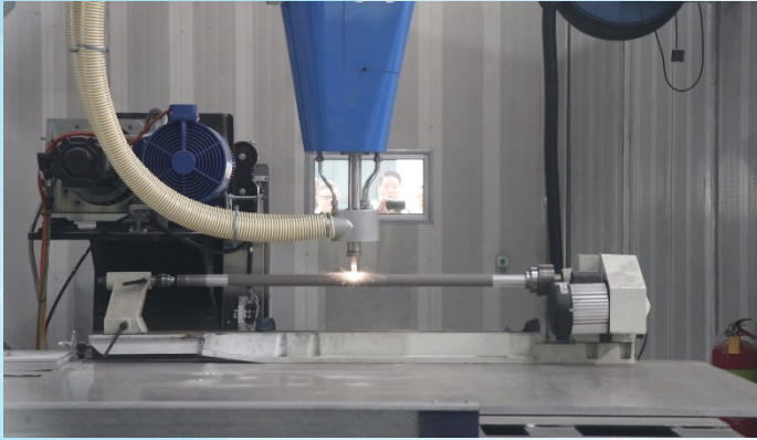
Titomic Kinetic Fusion™ demonstrates mandrel deposition at Titomic R&D Production Centre in Melbourne yesterday.
