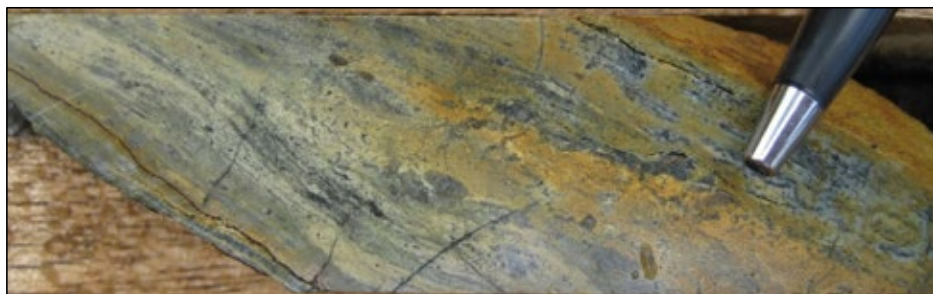
Figure 2-5: Drill core of schist from JHD09 at 43.6–48.5 m which has been overprinted by late fault movement at silicification
