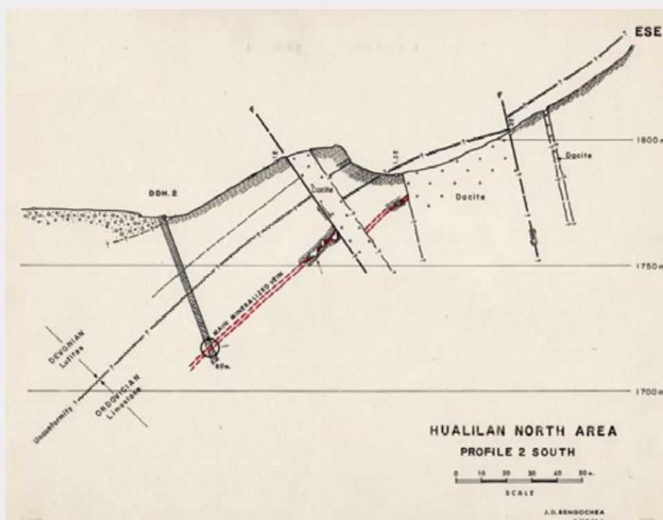
Historical Cross Section Cerro Norte (After Minera Aguilar S.A.)
