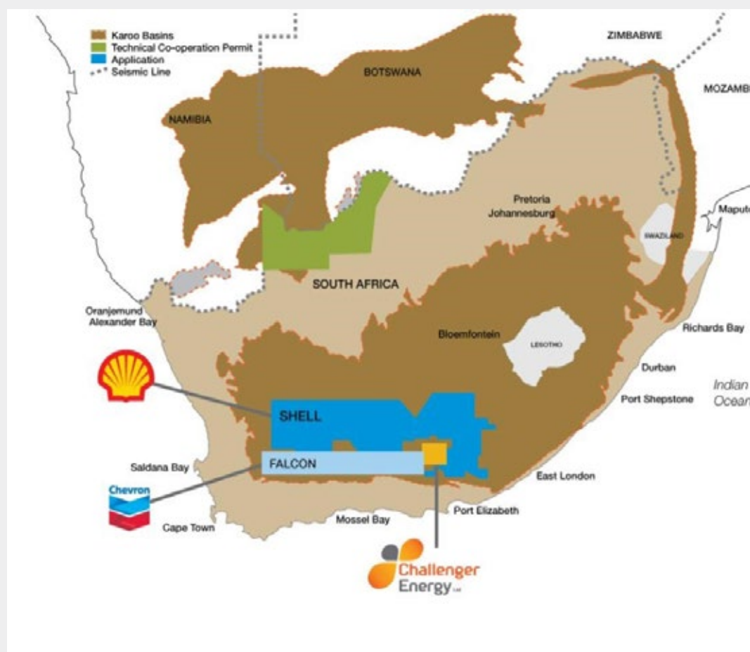
Karoo Shale gas location map
