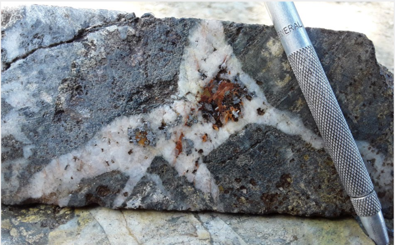
Core Photo JDH-06 (148m)
