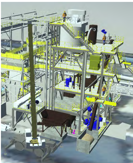
FGO Flash Flotation & Cyclone Efficiency
