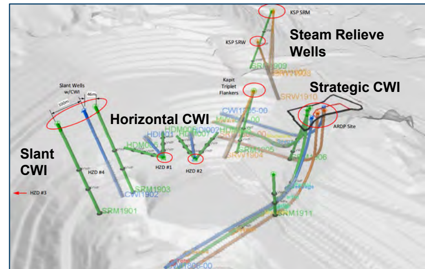
Diagram of directional drilling
