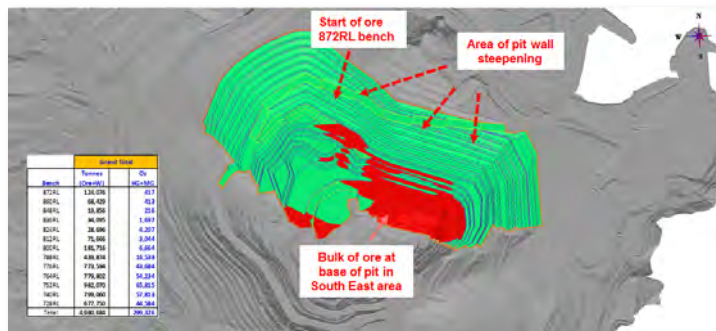
PH14 Design Ver5.0 with Total Material Gained
