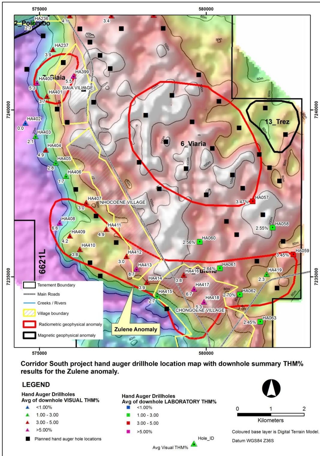
Figure 1: Location map of the Zulene anomaly (Corridor South project 6621L) hand auger drillholes reported in this update and reported previously, showing summary visual estimated data for THM grades. Drillhole names are shortened (e.g., 'HA402') for presentation, but are prefixed by '20CS' in the database.
