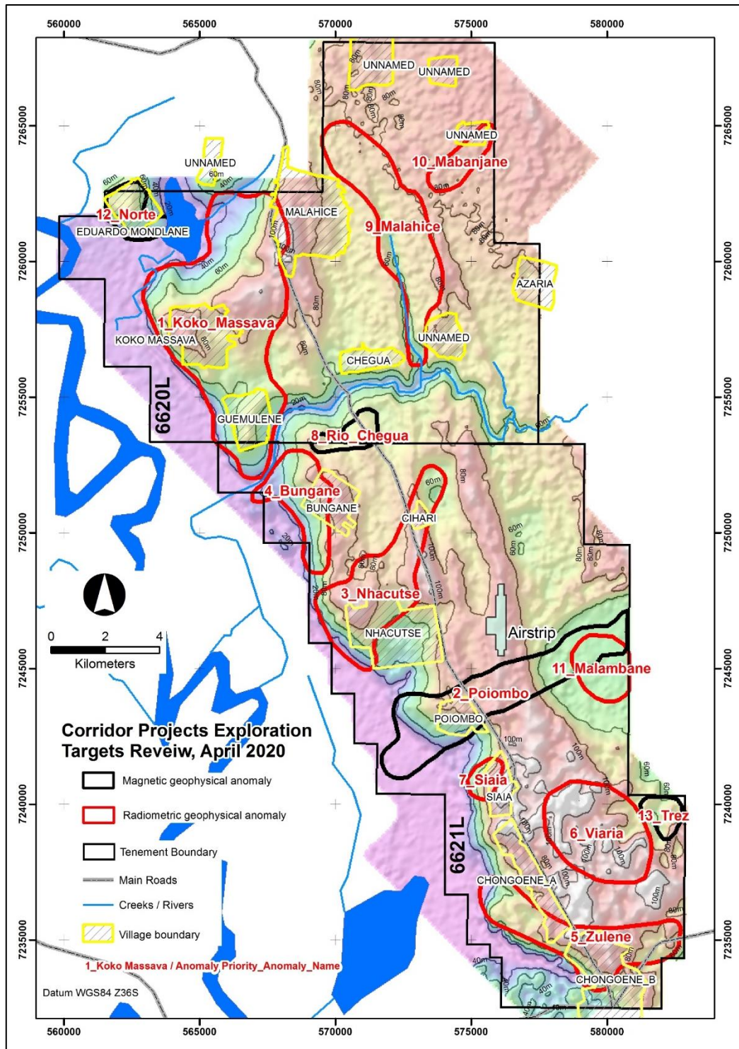
Figure 3: Map of the Corridor Central (6620L) and Corridor South (6621L) projects showing prioritised geophysical anomalies based on a review in April 2020 (refer announcement 12 May 2020).
