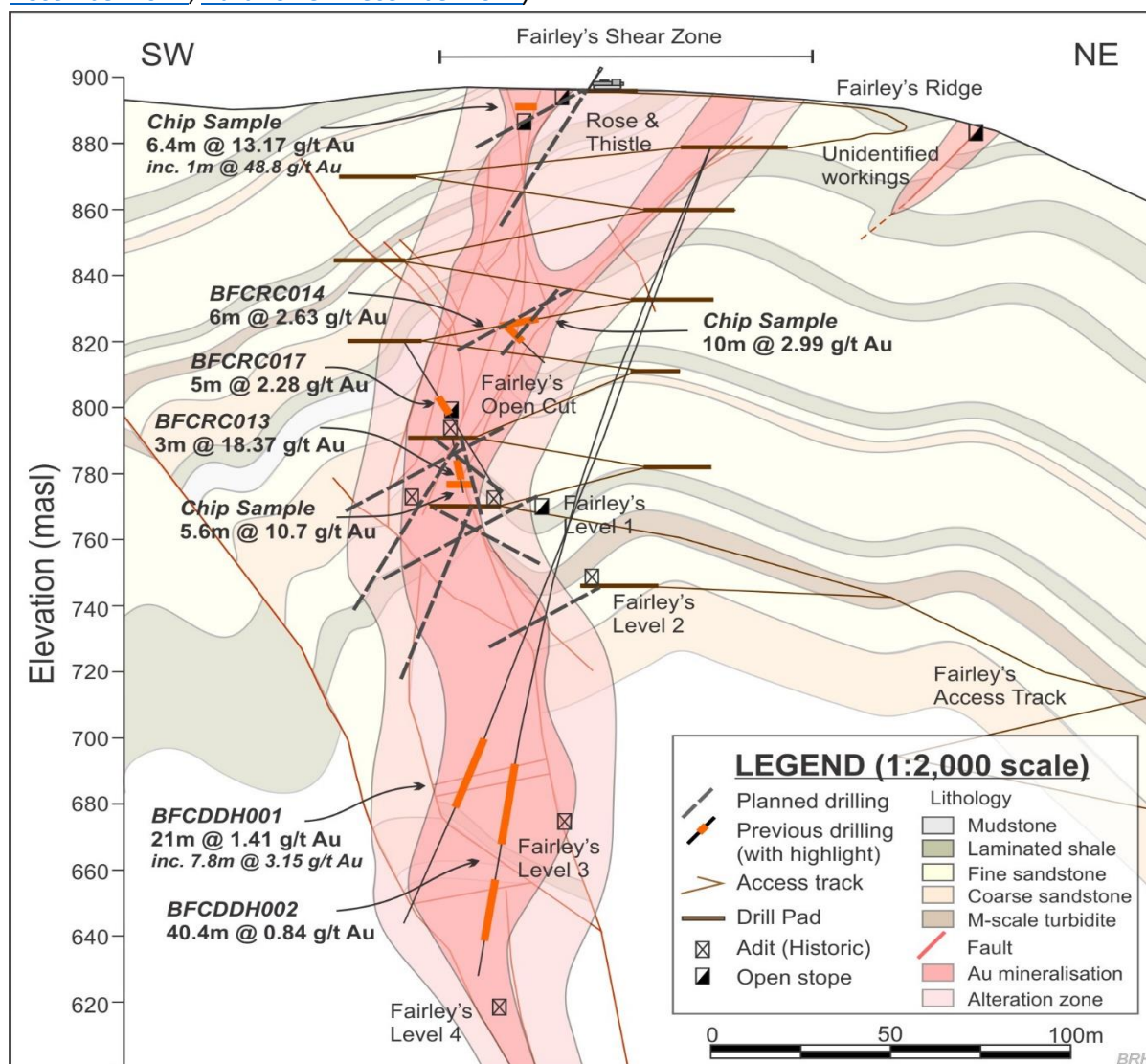
Figure 1: Cross-section of targeted mineralisation at Fairley's. Selected highlights from previous drilling ( Dart ASX 15 December 2008 , Dart ASX 31 December 2008 ) and chip sampling shown ( Dart ASX December 2019 ; Dart ASX February 2020 ). Note that cross section (B) is compiled from approximately 150m of transposed data. See Figure 3 for map of planned drill holes.
