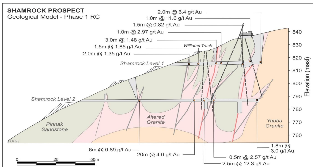
Figure 2: Cross-section through the Shamrock prospect showing sampling highlights and the conceptual geological model for altered granite mineralisation in the Sandy Creek Goldfield. High-grade silica-gold mineralisation is present along narrow veins (red lines), whereas granite intrusion and subsequent hydrothermal alteration has exploited fractures (grey lines), resulting in an inconsistent distribution of altered, gold mineralised granite. Section is oriented northeast-southwest and drawn to scale (1:1000).
