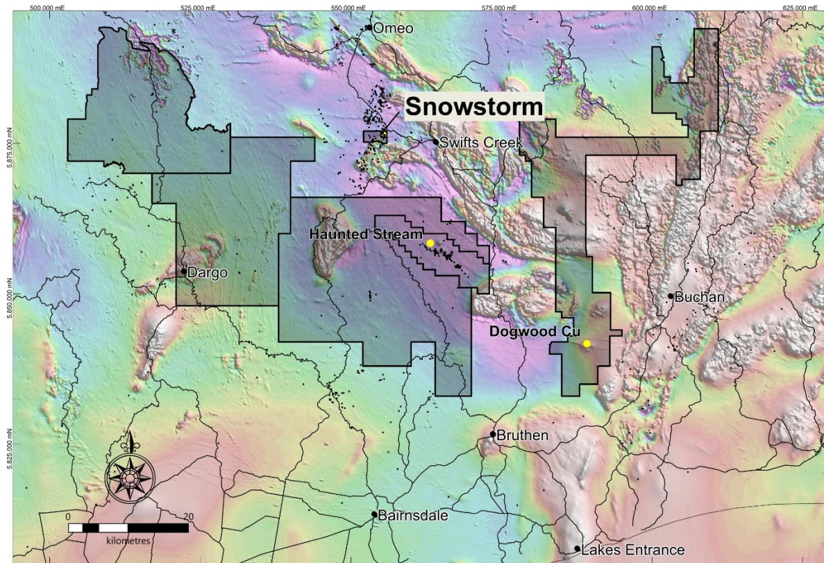
Figure 4. TMI magnetic image with the VicGold Tenement application area, including the new Snowstorm Project location. (Co-ords MGA94, Zone 55)
