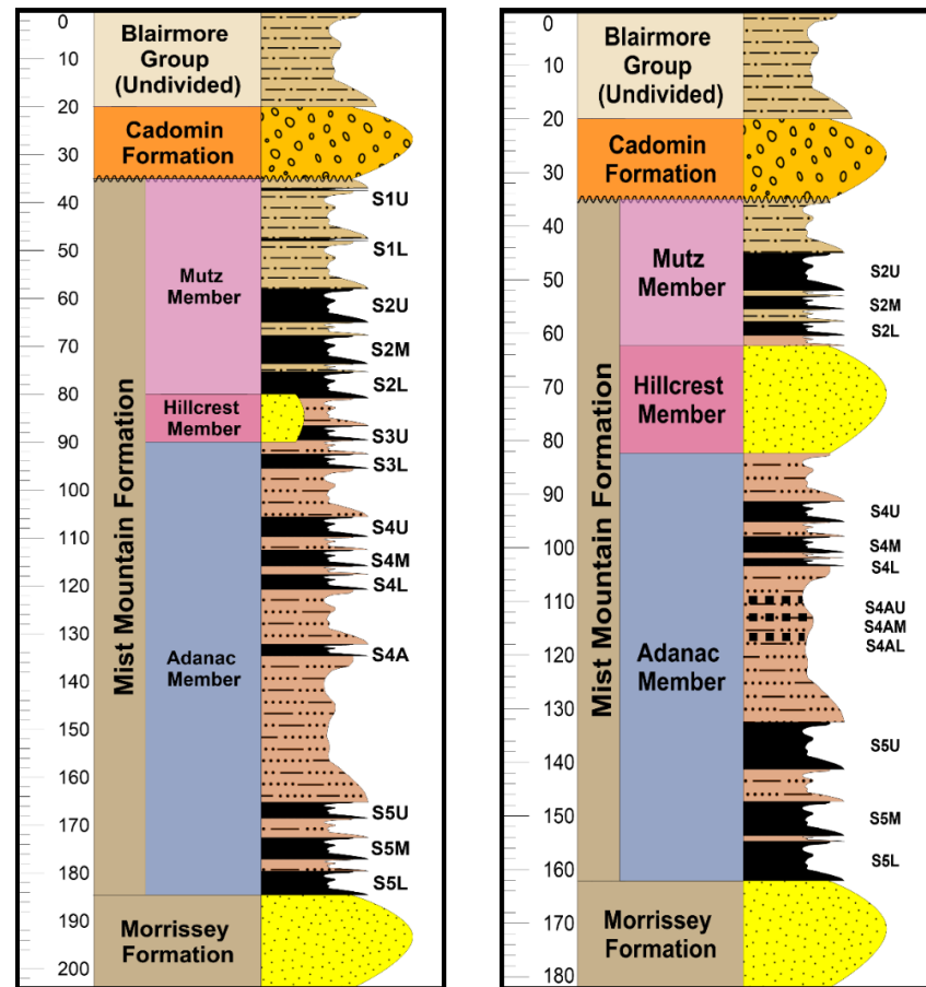
Chinook South (left) and Chinook Vicary (right) Stratigraphy
