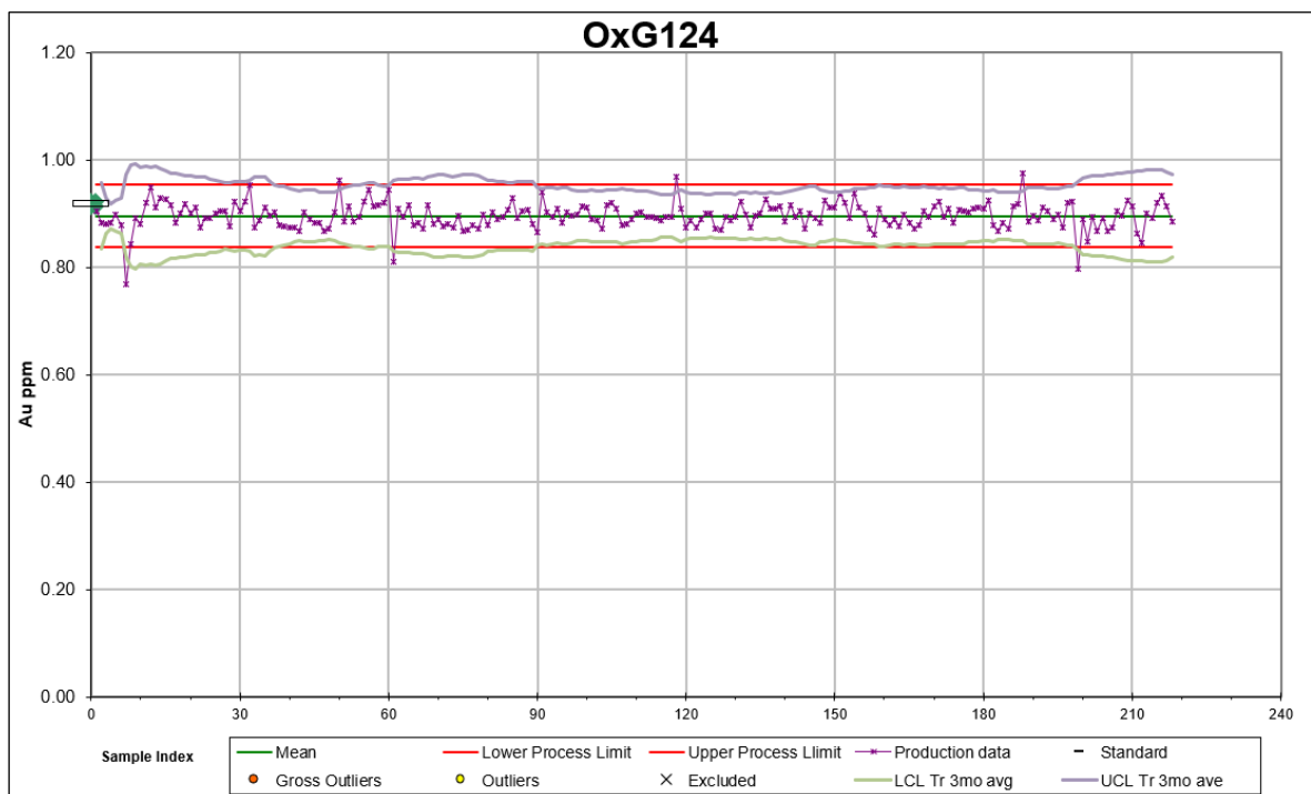
Figure 12-6: July 2017-Current, Control Chart, OxG124 (n=218)
