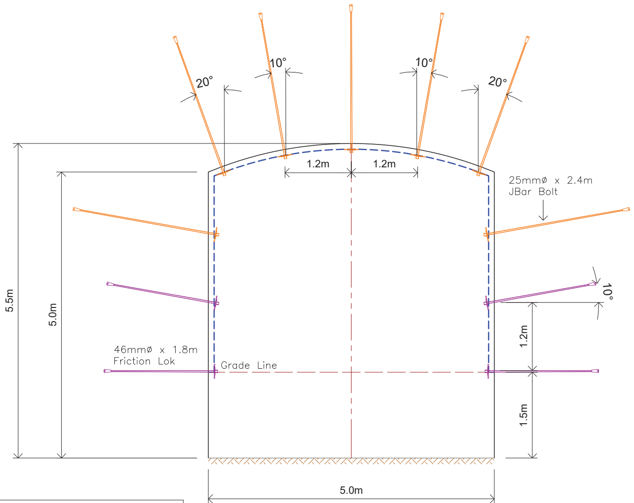
DRIVE DESIGN (FRONT VIEW)
