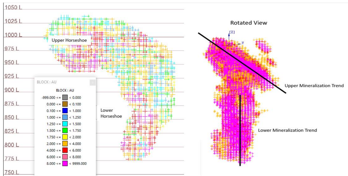
Figure 16-11: Horseshoe Upper and Lower Mineralized Zones
