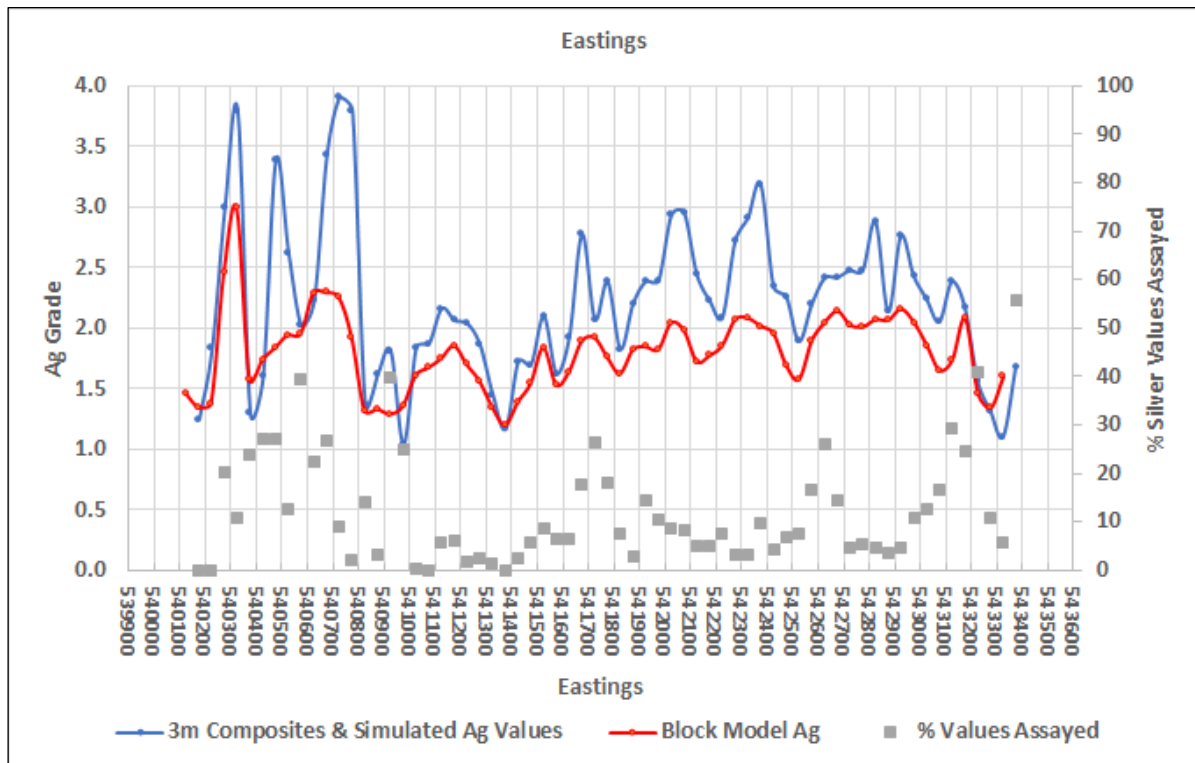
Figure 14-6: Swath Plot with Mean Composite Silver Grade vs HA0520OLM Block Values
