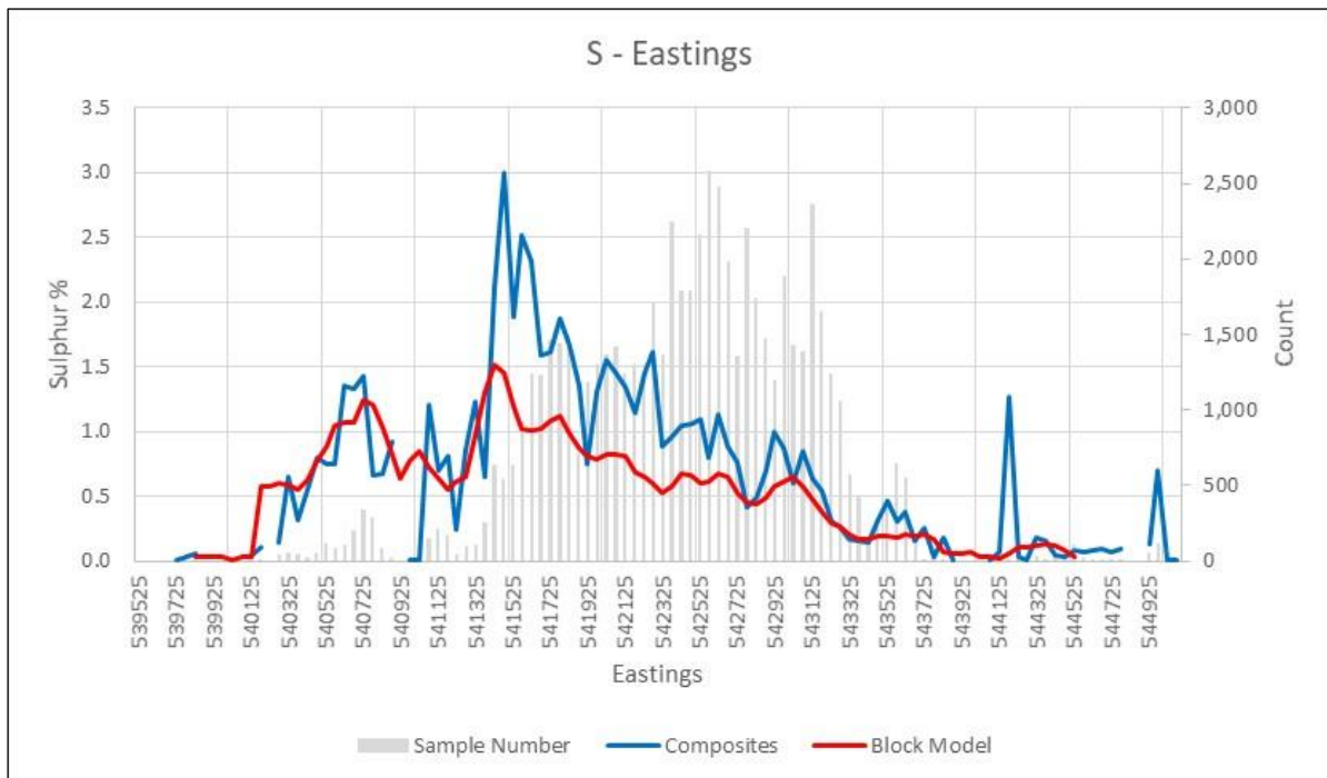
Figure 14-5: Swath Plot with Mean Composite Sulfur Grade vs HA0520OLM Block Values
