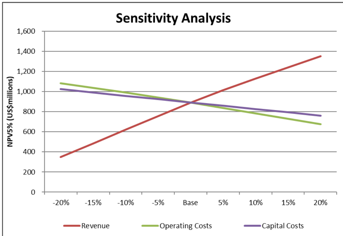
Figure 22-6: Operational Sensitivity Analysis
