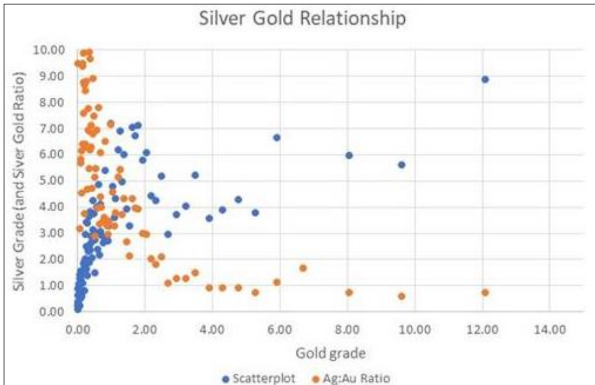
Figure 14-2: Silver Gold Relationship for Gold Ranked Percentile Averaged Grades
