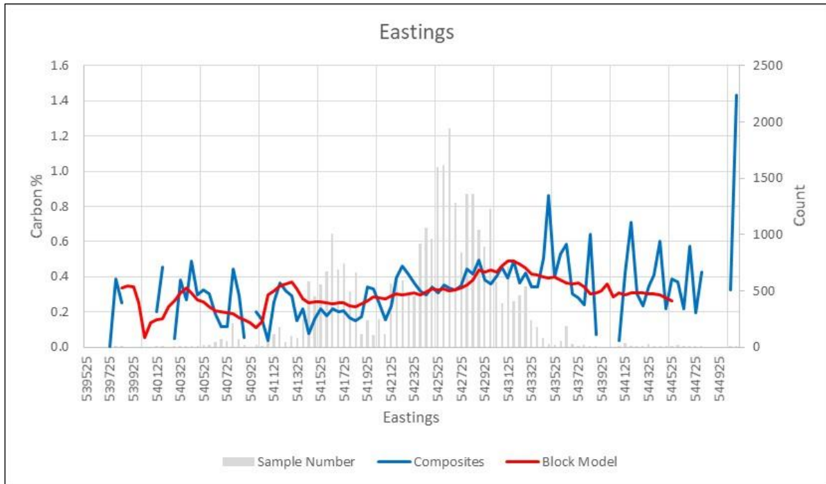
Figure 14-4: Swath Plot with Mean Composite Carbon Grade vs HA0520OLM Block Values
