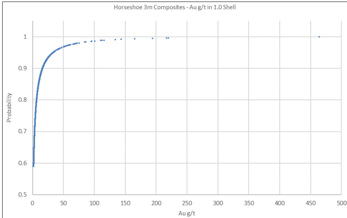
Figure 14-7: Log Normal Cumulative Distribution Plot of Gold Assays Above 2 g/t
