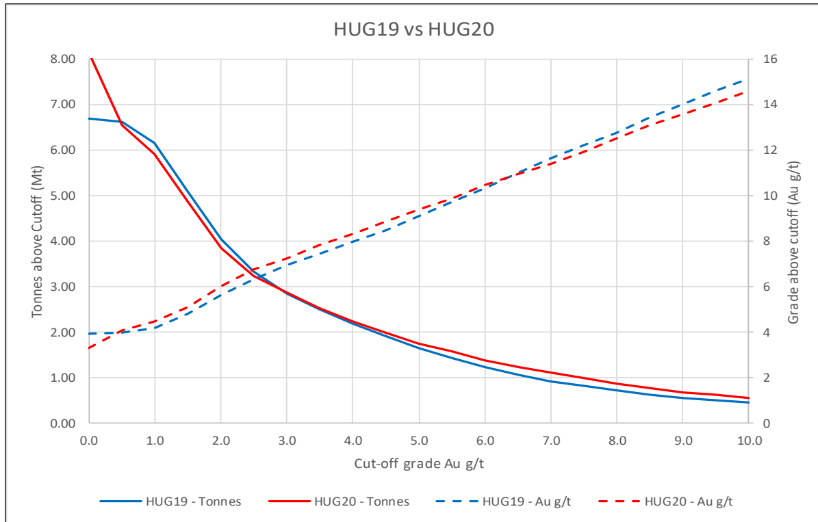
Figure 14-8: Global Grade Tonnage Comparison between 2019 and 2020 Models
