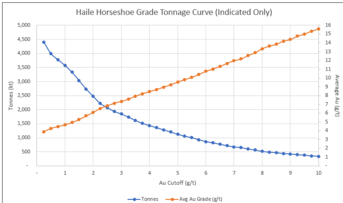
Figure 16-13: Horseshoe Underground Model Grade/Tonne Curve Based on Au Cut-off
