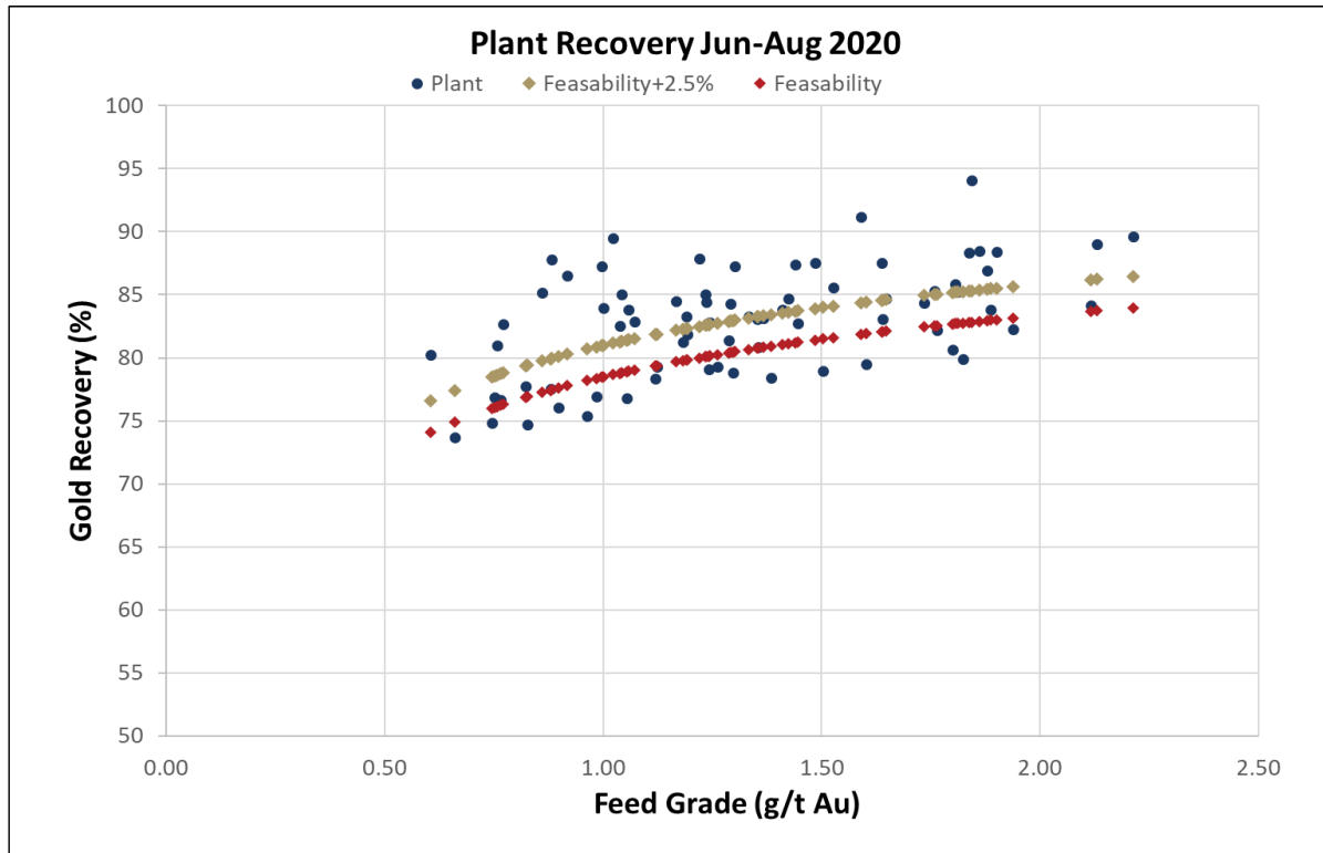
Figure 13-3: Plant Gold Recovery Performance Jun-Aug 2020
