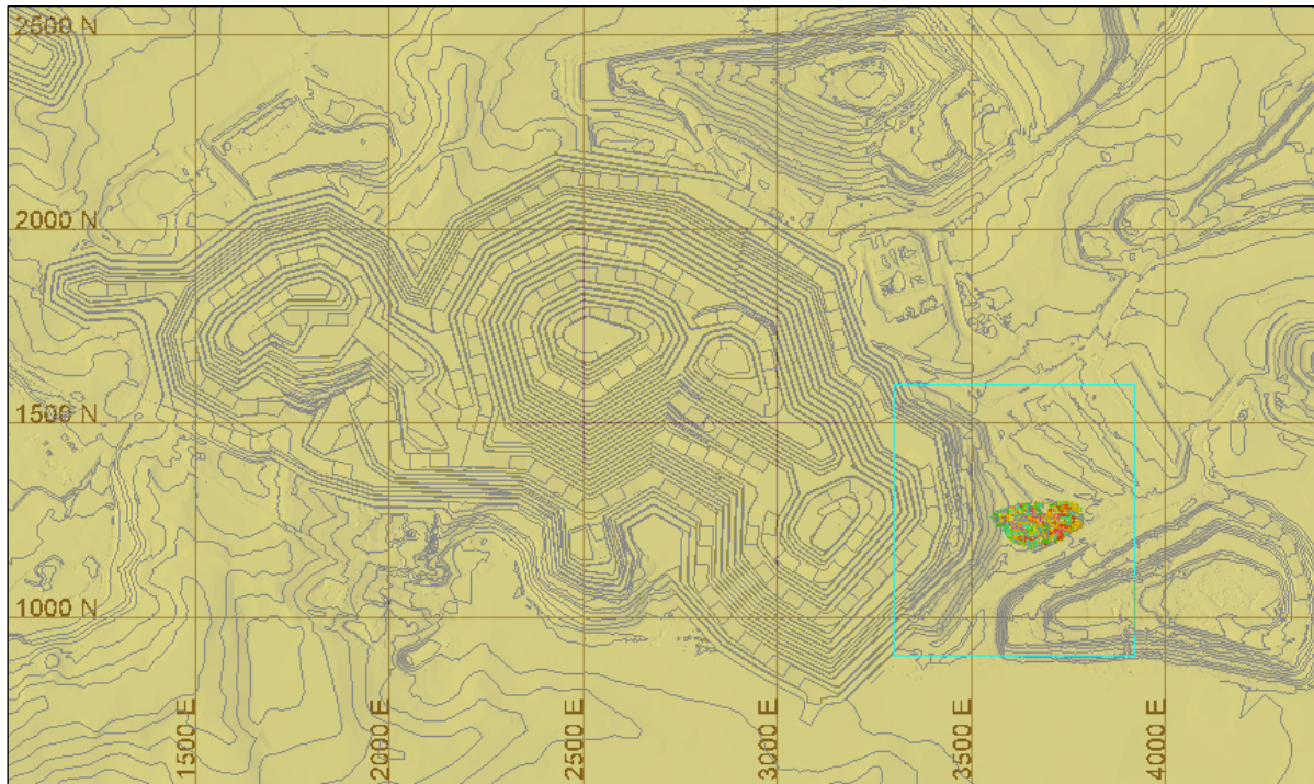
Figure 16-12: Haile Underground Block Model and Mineralization Extents
