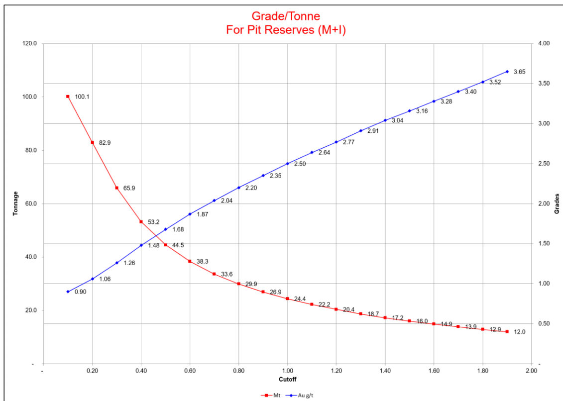
Figure 16-7: Grade Tonnage Curve within Reserve Pit (Measured and Indicated Material)
