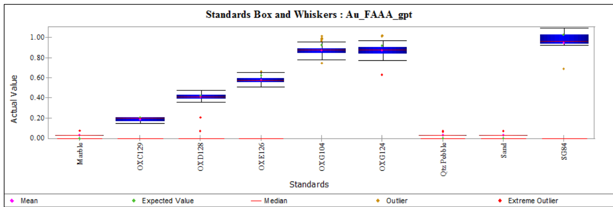
Figure 12-1: Box and Whiskers Plots for Horseshoe 2016 Standards and Blanks
