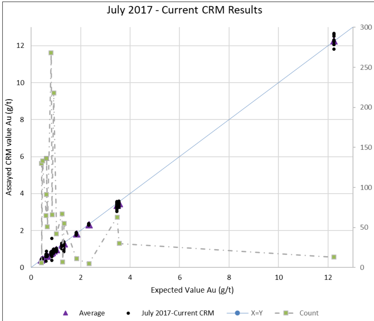
Figure 12-3: July 2017-Current CRM Analyses versus Expected Value (n=1,457)
