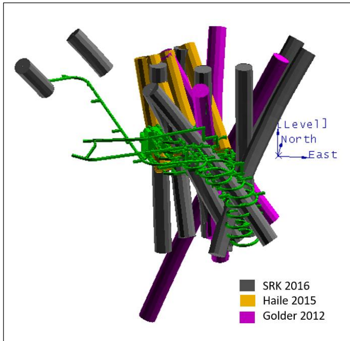
Figure 16-14: Horseshoe 2020 Underground Workings with As-Drilled Characterization Core Holes
