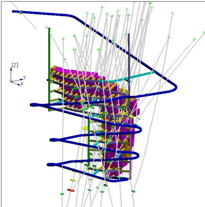
Figure 16-26: Location of PEA and FS Geochemical Samples Color Coded using Haile Criteria
