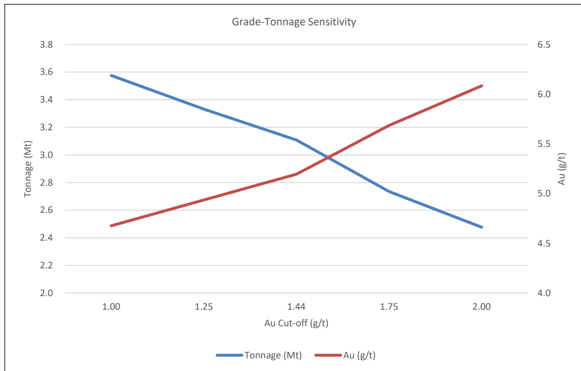
Figure 14-14 Sensitivity of Indicated Resource Tonnes and Grade to Cut-off
