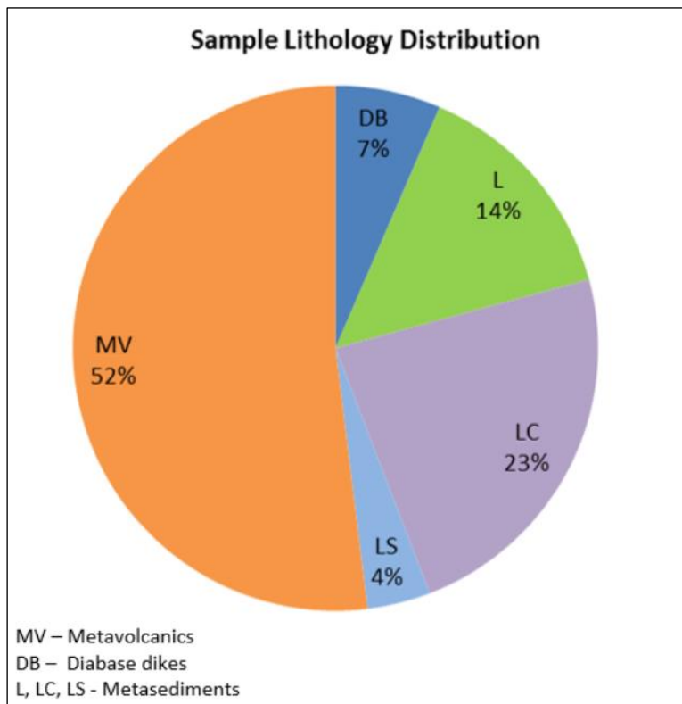
Figure 16-23: Horseshoe FS/PEA Lithological Distribution of Samples
