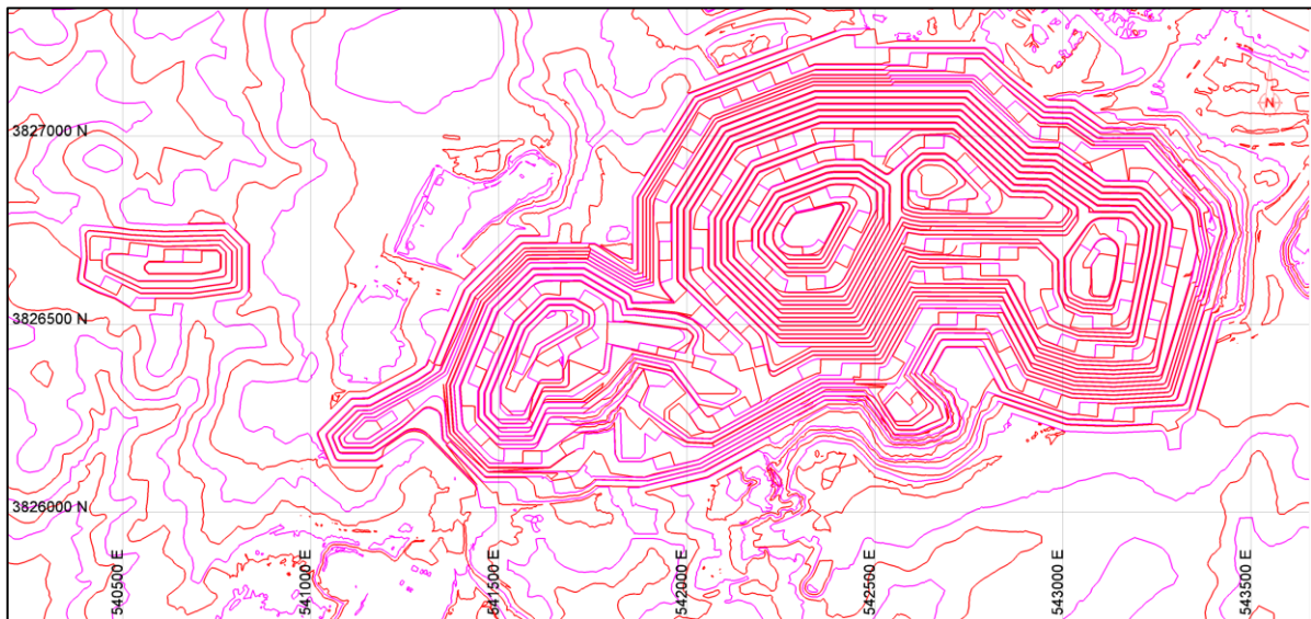
Figure 16-6: LoM Pit Design
