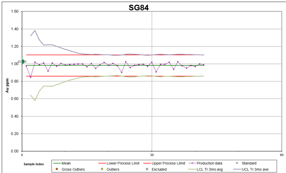
Figure 12-7: July 2017-Current, Control Chart, SG84 (n=42)
