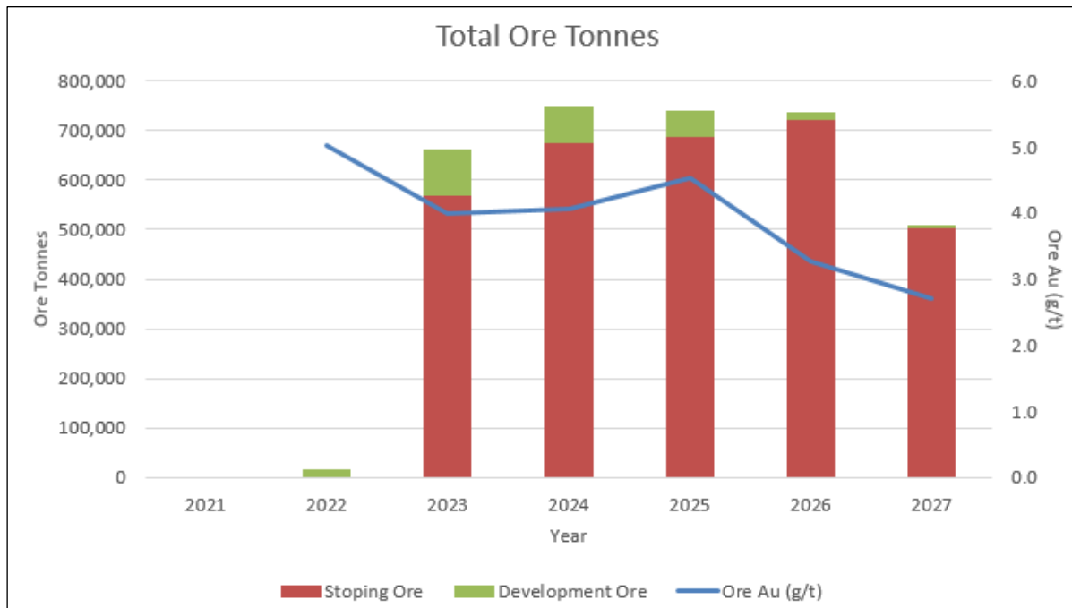
Figure 16-34: Ore Tonnes by Activity Type
