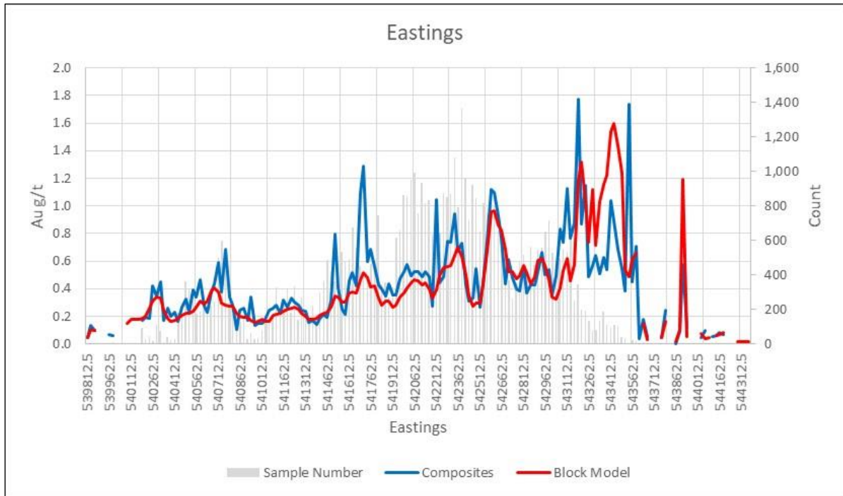
Figure 14-3: Swath Plot with Mean Composite Gold Grade vs HA0520OLM Block Values
