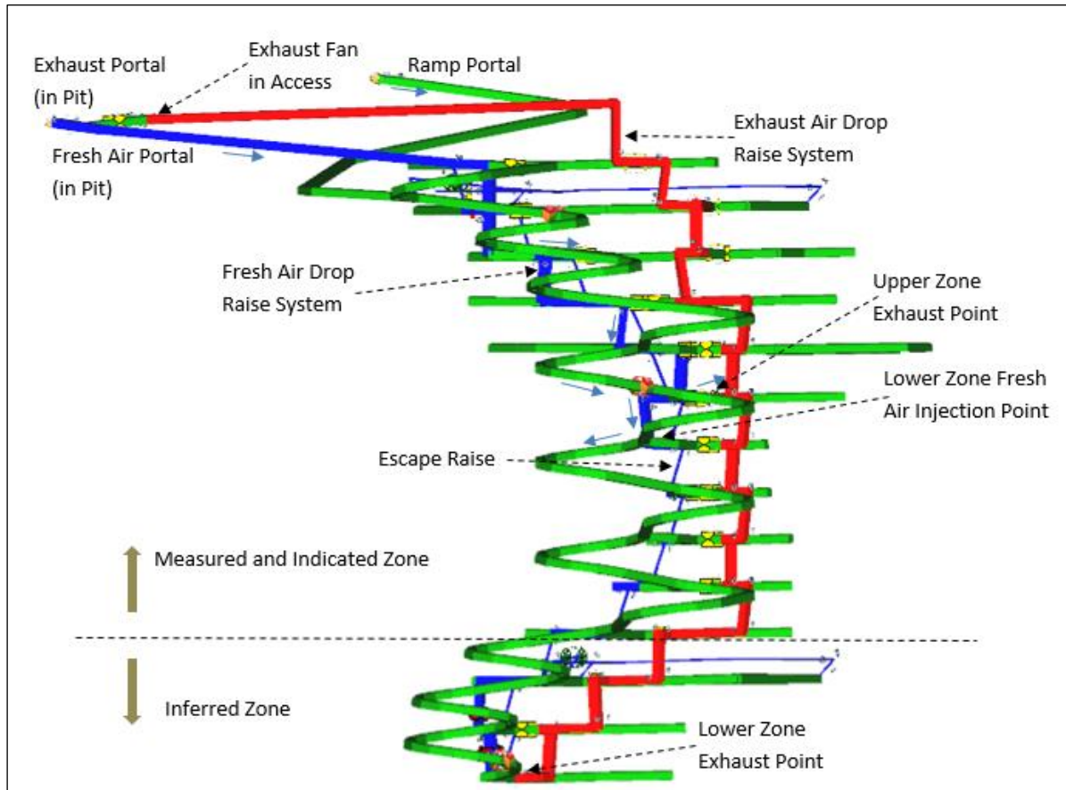
Figure 16-40: Ventilation System Layout
