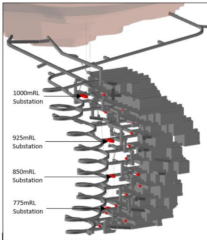
Figure 16-43: Electrical System Layout
