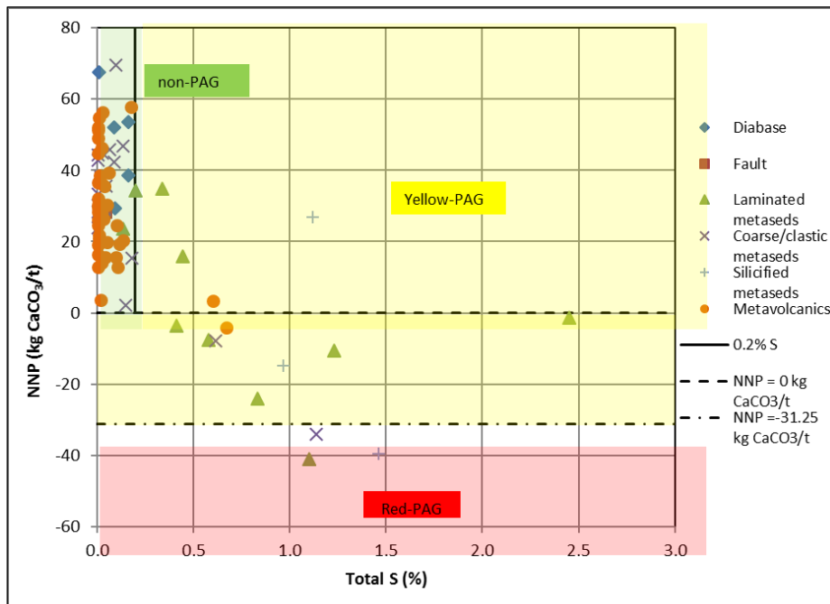
Figure 16-25: NNP vs. Total Sulfur for Horseshoe Development Rock
