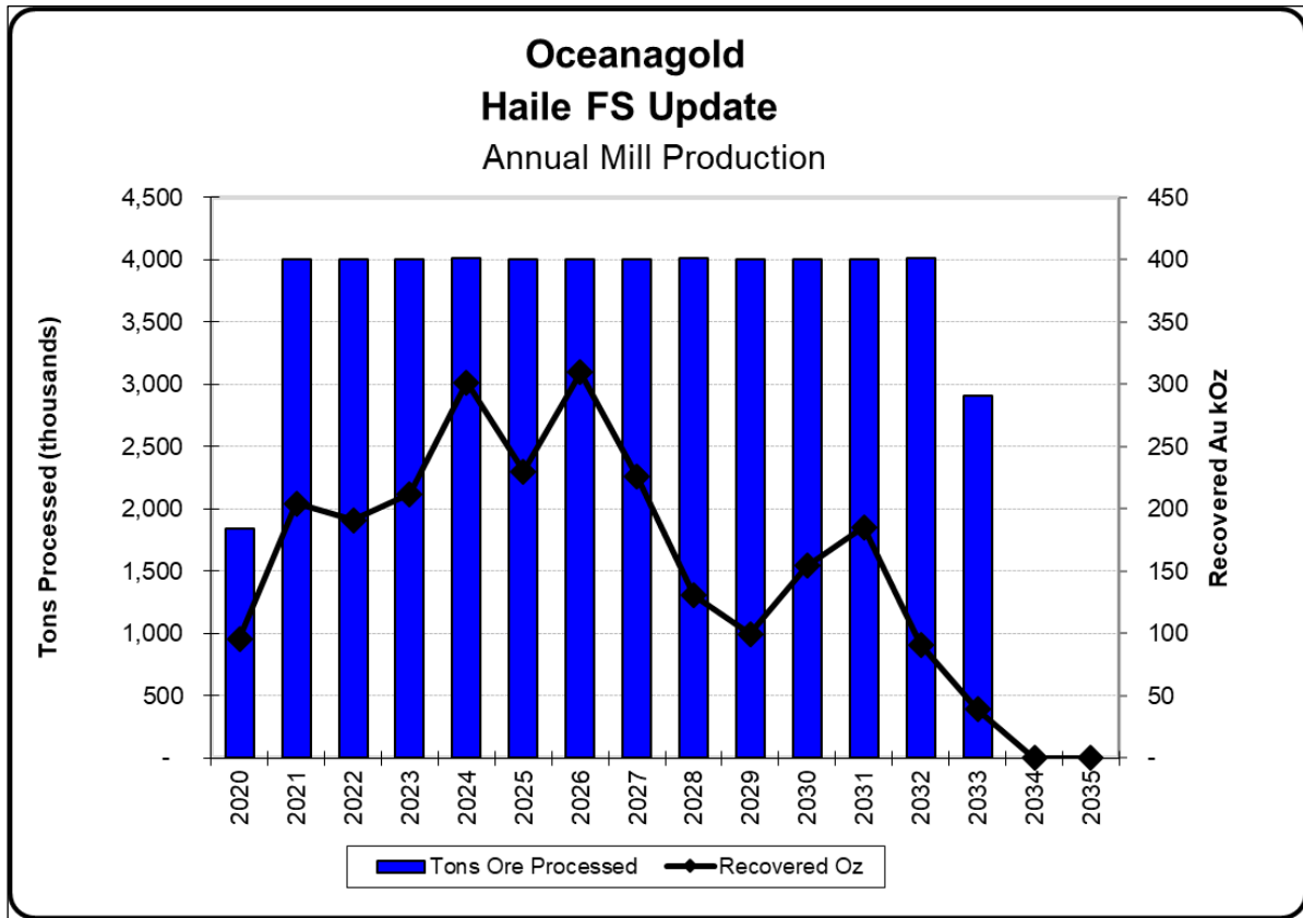
Figure 22-3: Annual Process Plant Production
