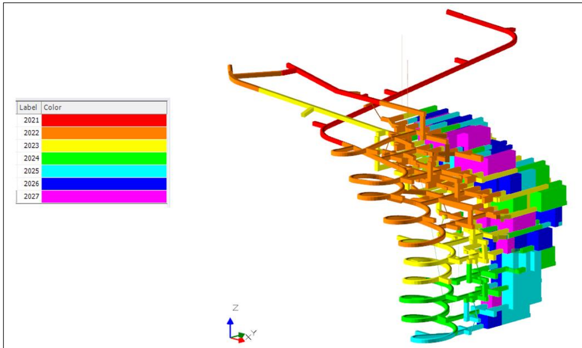
Figure 16-33: Mine Production Schedule Colored by Year (looking NW)
