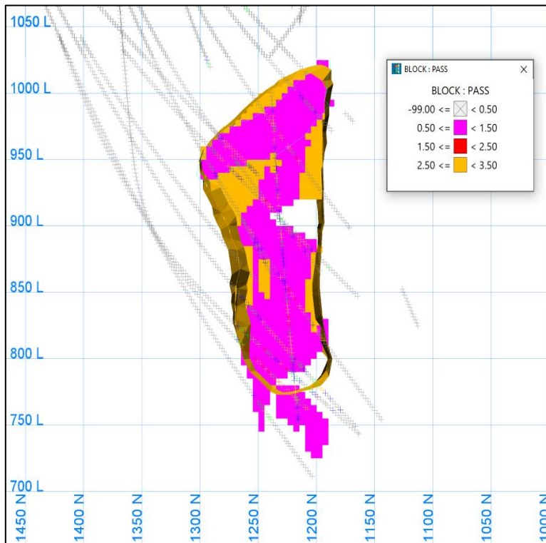
Figure 14-12: Representative Cross Section Showing Indicated Wireframe around Pass 1 Estimated Blocks (Viewing N90°E)
