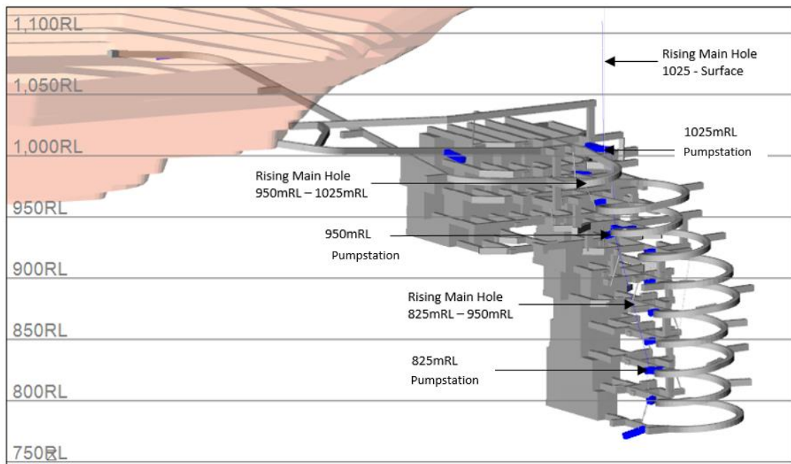
Figure 16-41: Dewatering System Layout
