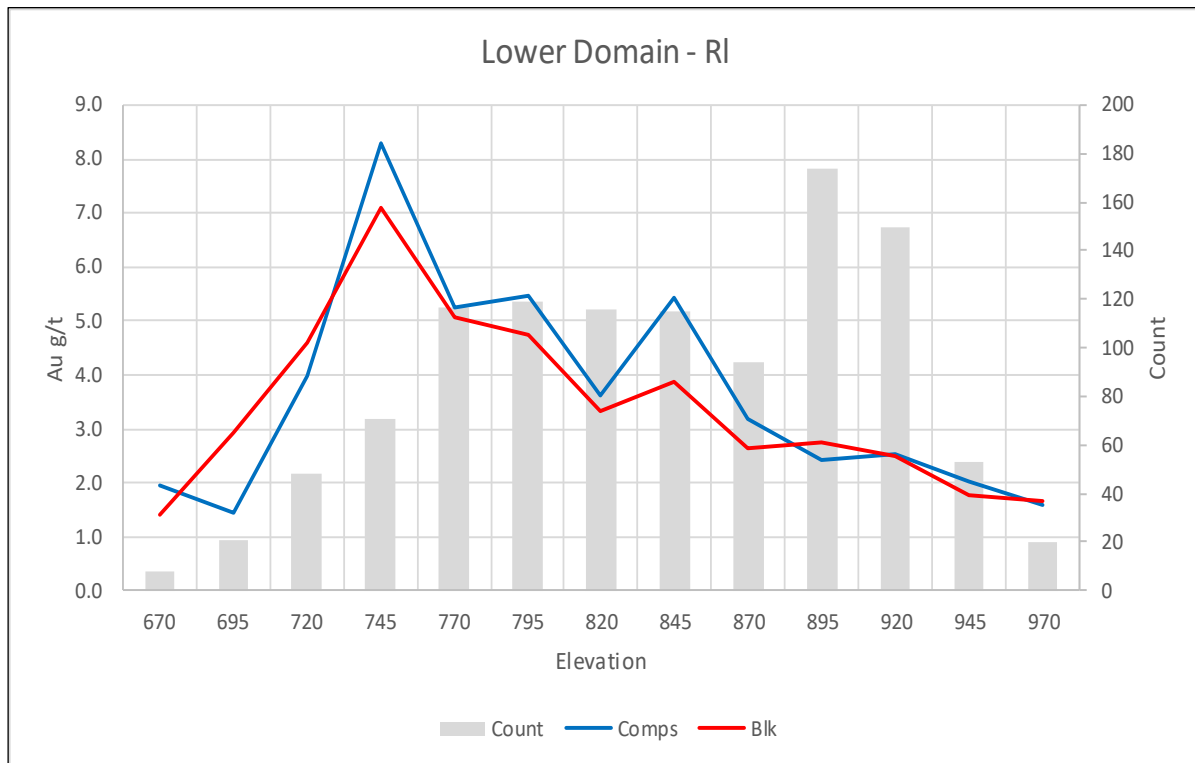
Figure 14-10: Lower Domain RI Swath Plot
