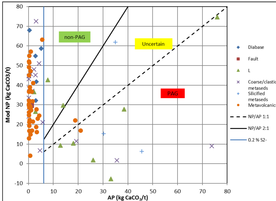
Figure 16-24: NP/AP for Horseshoe Development Rock
