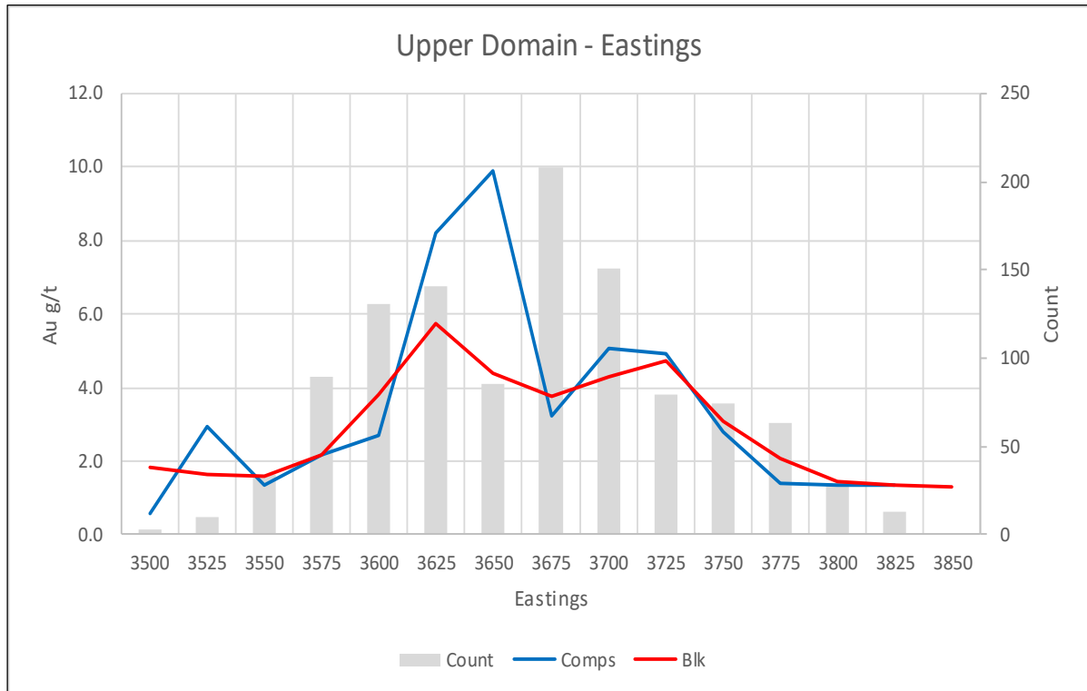
Figure 14-9: Upper Domain Easting Swath Plot
