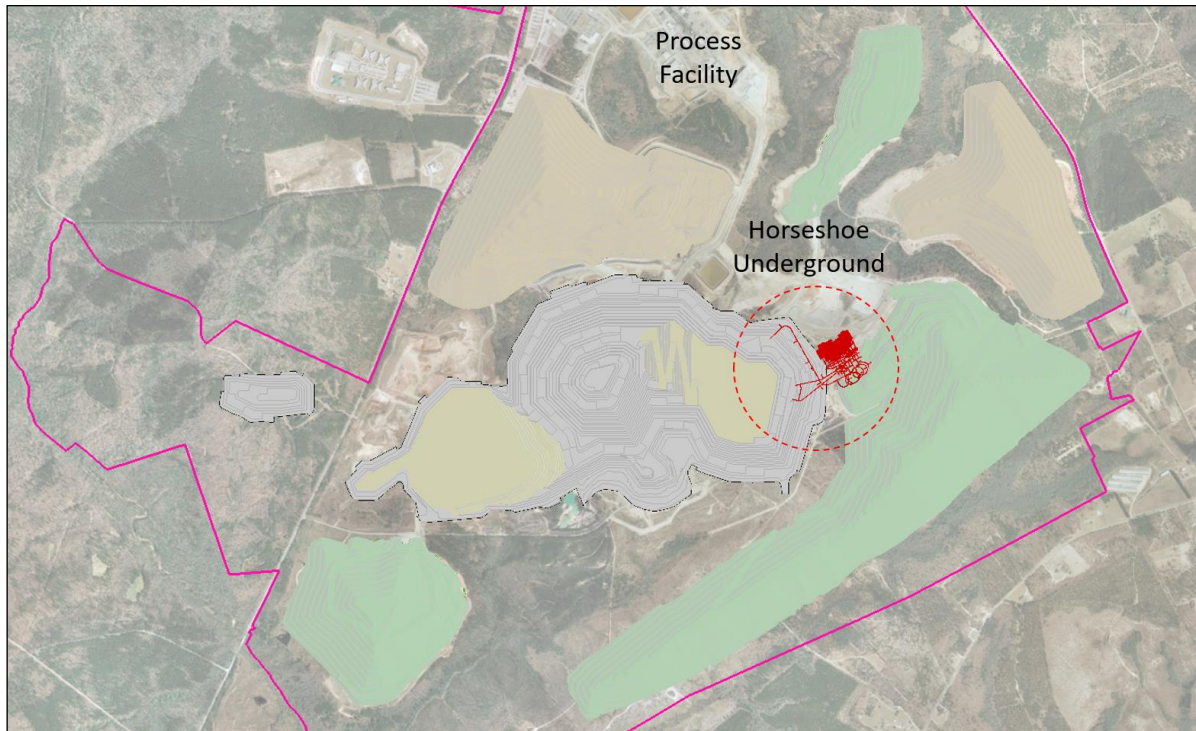
Figure 15-1: General Site Layout and Location of the UG Reserve Area
