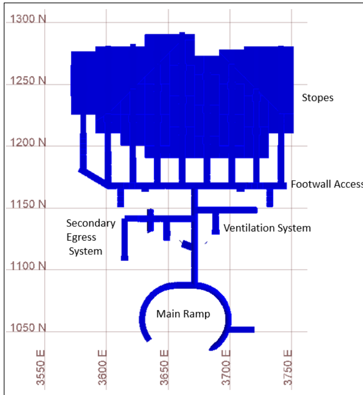
Figure 16-30: Typical Level Section
