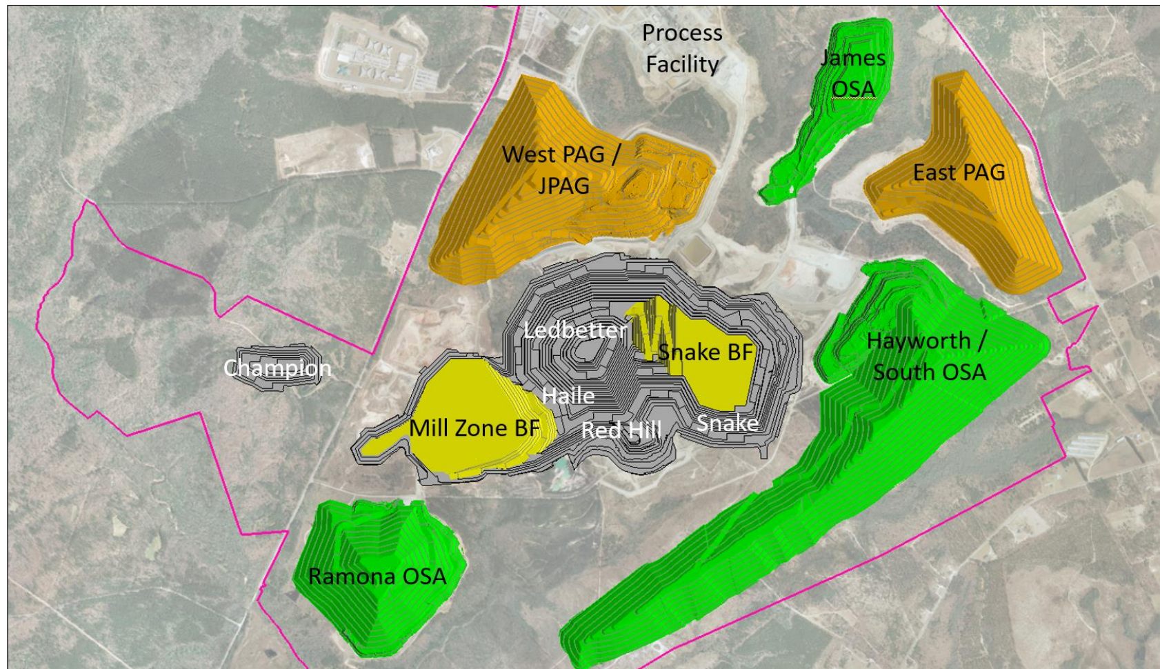
Figure 16-8: Final Pit Design and Ultimate Overburden Storage Site Plan
