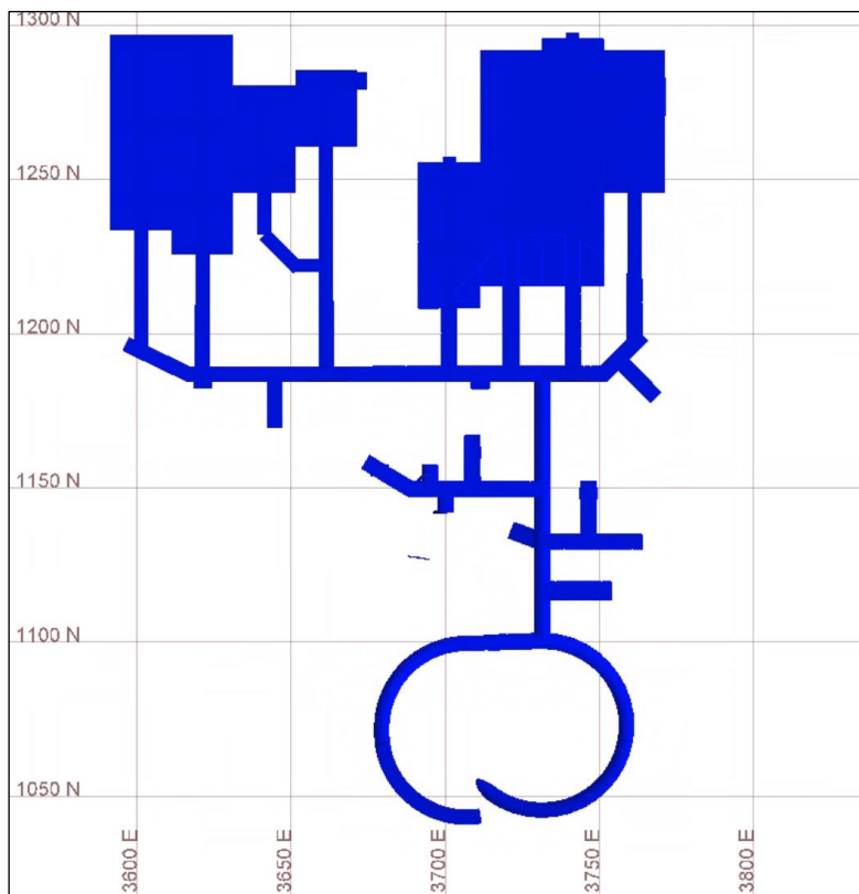
Figure 16-18: Plan View of 930 Level Showing Proximity of Footwall Access Drifts to Planned Stopes
