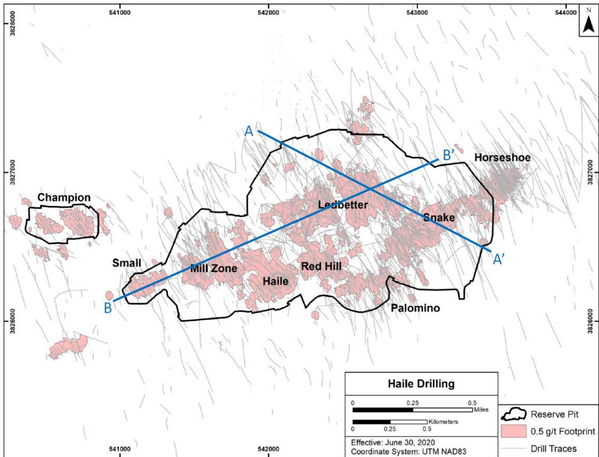
Figure 7-5: Plan View of Drillholes used for Resource Estimation, Gold Mineralization, and EOY 2019 Reserve Pit Limit (Sections A-A' and B-B' are Presented in Figure 7-6)
