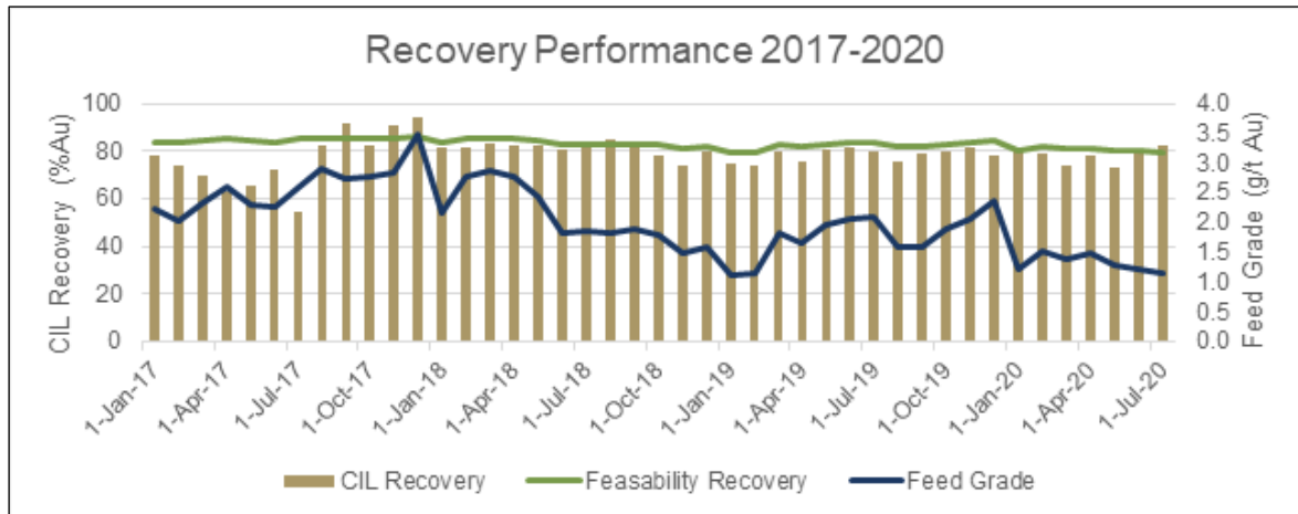
Figure 17-5: Gold Recovery Performance Since Startup
