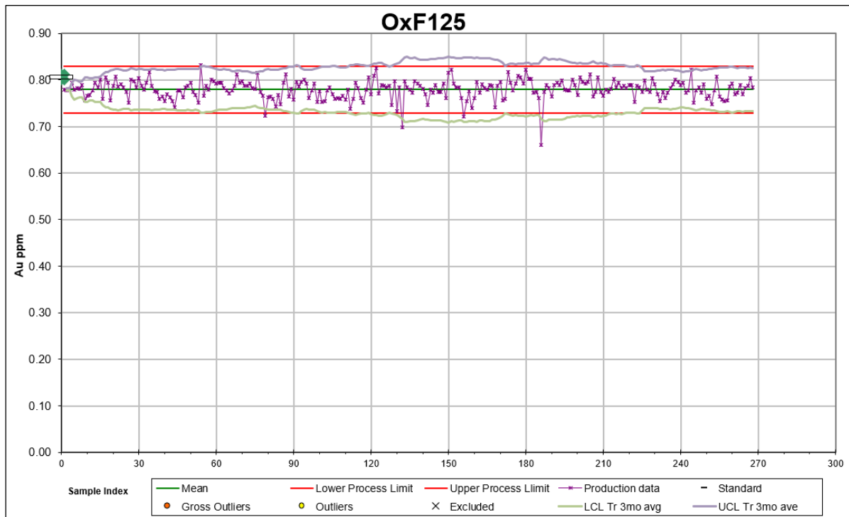
Figure 12-5: July 2017-Current, Control Chart, OxF125 (n=268)
