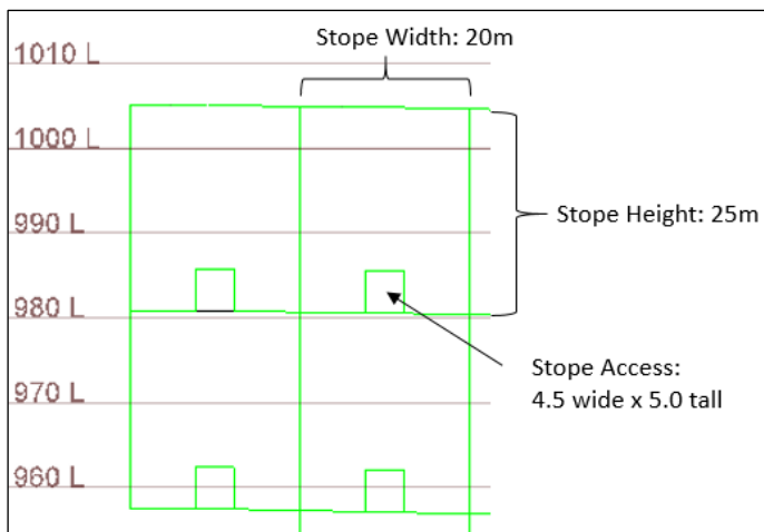
Figure 16-28: Stope Cross Section
