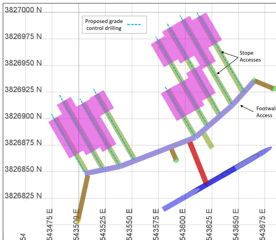
Figure 16-38: Level Section Showing Planned Diamond Drilling from Footwall Access Drifts
