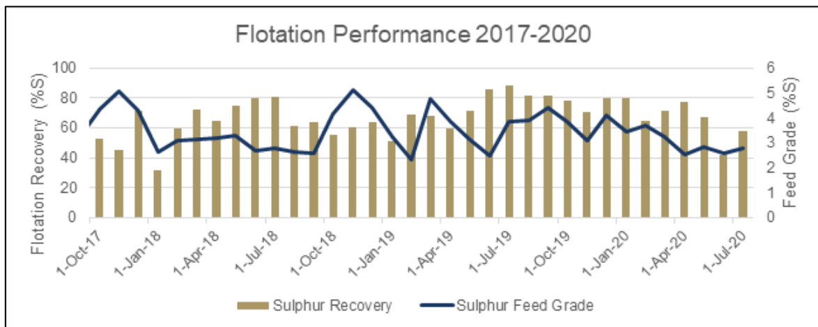
Figure 17-4: Flotation Circuit Recovery
