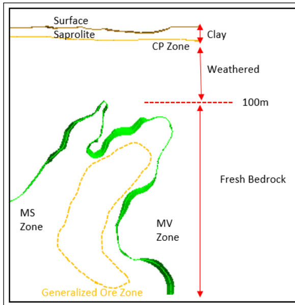
Figure 16-15: Geotechnical Model Cross Section (Looking NE)
