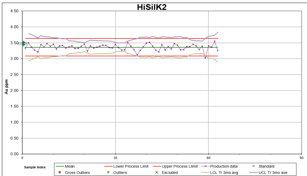
Figure 12-8: July 2017-Current, Control Chart, HiSilK2 (n=63)
