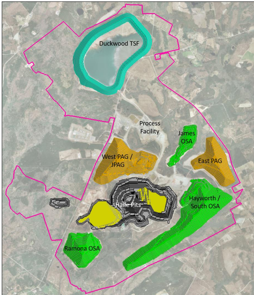
Figure 1-1: Final Pit Design and Site Layout
