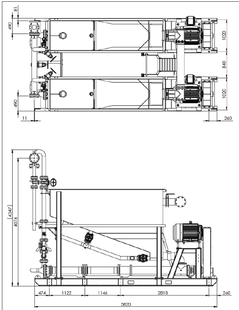
Figure 16-42: Portable Pumping Skids
