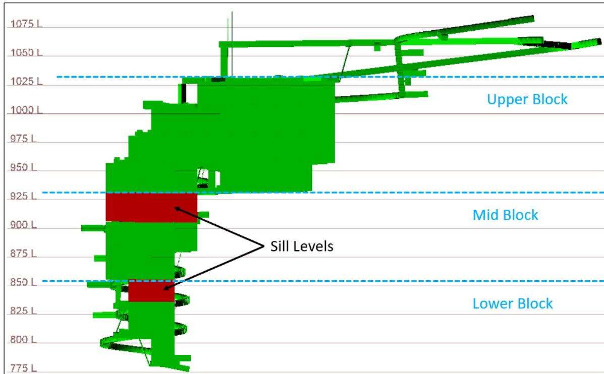
Figure 15-2: UG Design Sill Levels (local grid)
