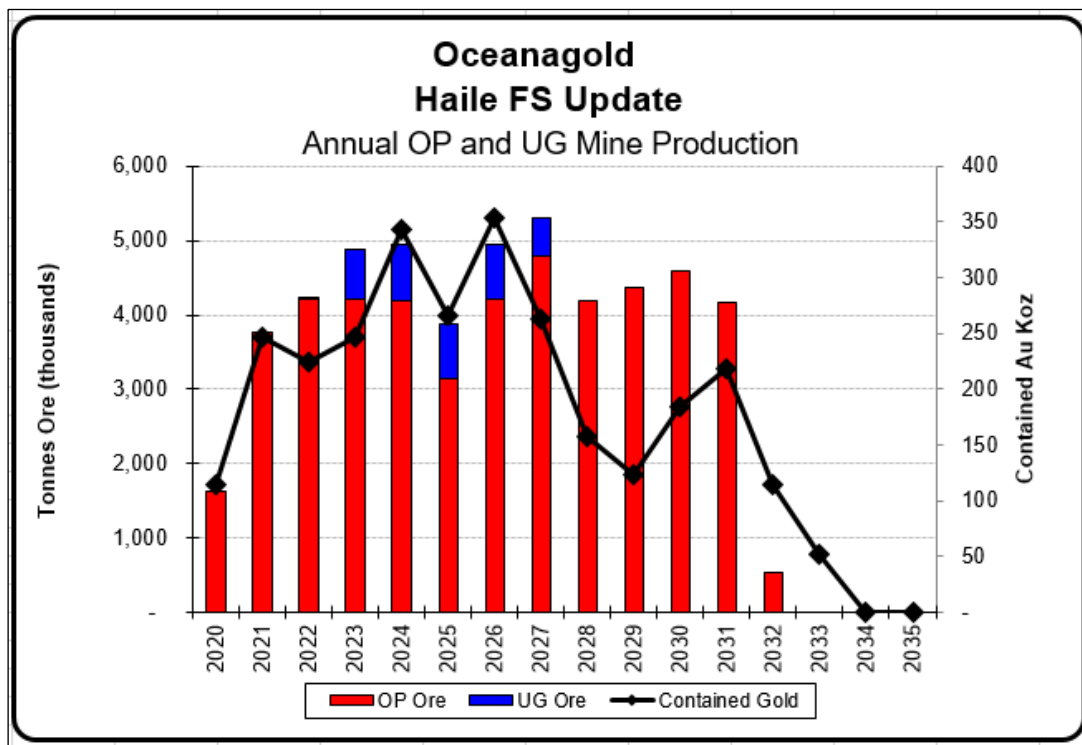
Figure 16-44: Combined Open Pit and Underground Production
