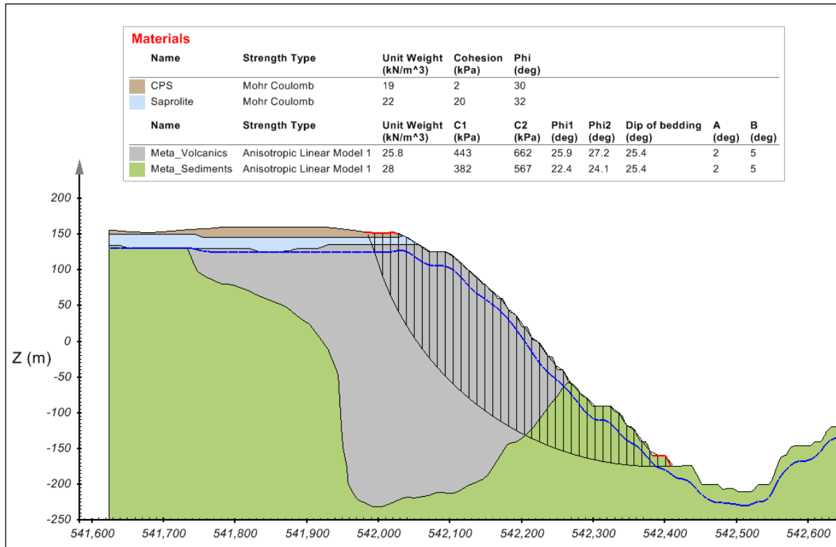
Figure 16-4: Section View Through Critical Mass of 3D Overall Analysis of Northwest Corner of the Ledbetter Pit
