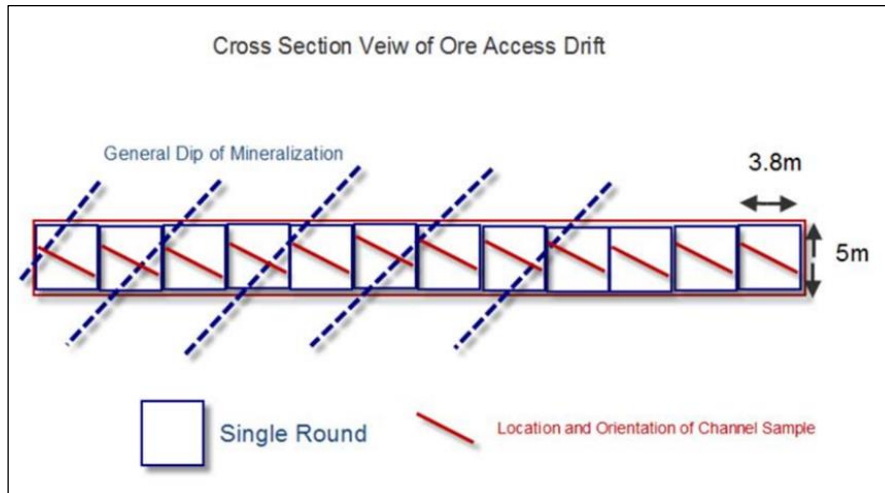
Figure 16-39: Cross Section View of Development Rounds and Proposed Channel Sampling Locations
