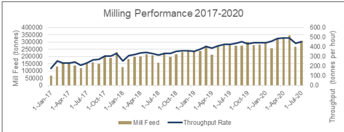
Figure 17-2: Mill Throughput Performance Since Startup
