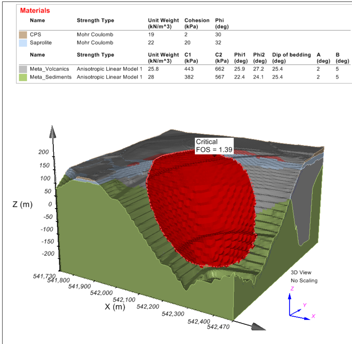
Figure 16-3: Example of 3D Overall Analysis: Northwest Corner of the Ledbetter Pit
