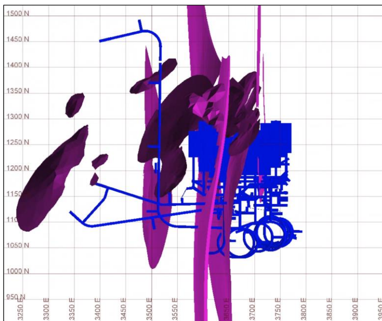
Figure 16-17: Plan View of Planned Workings Showing Dikes (local grid)
