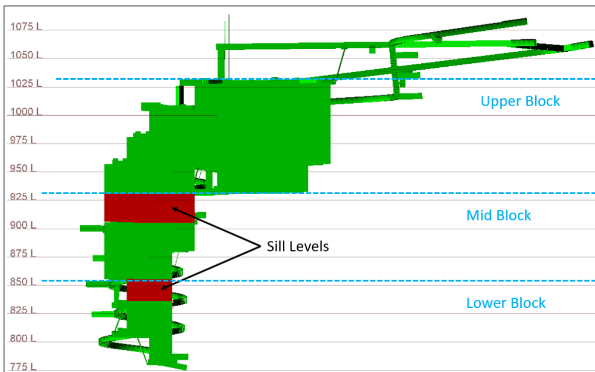
Figure 16-20: Sill Pillars (Red Stopes) to be Extracted Late in Mining Sequence
