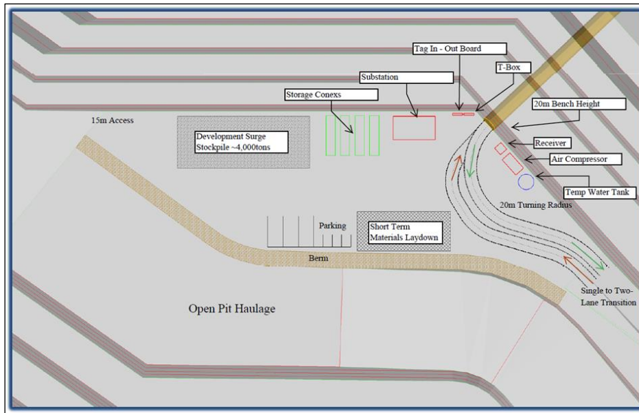
Figure 18-8: Production Portal Layout
