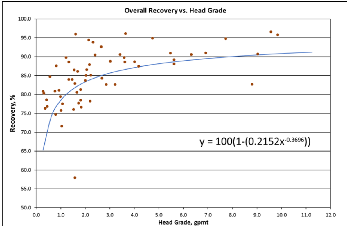
Figure 13-2: Overall Percent Recovery vs. Head Grade
