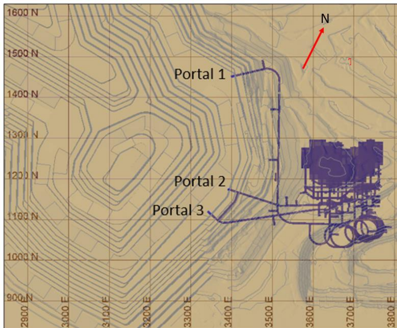
Figure 16-16: Snake Pit Showing Slopes Above Proposed Horseshoe UG Portal Locations
