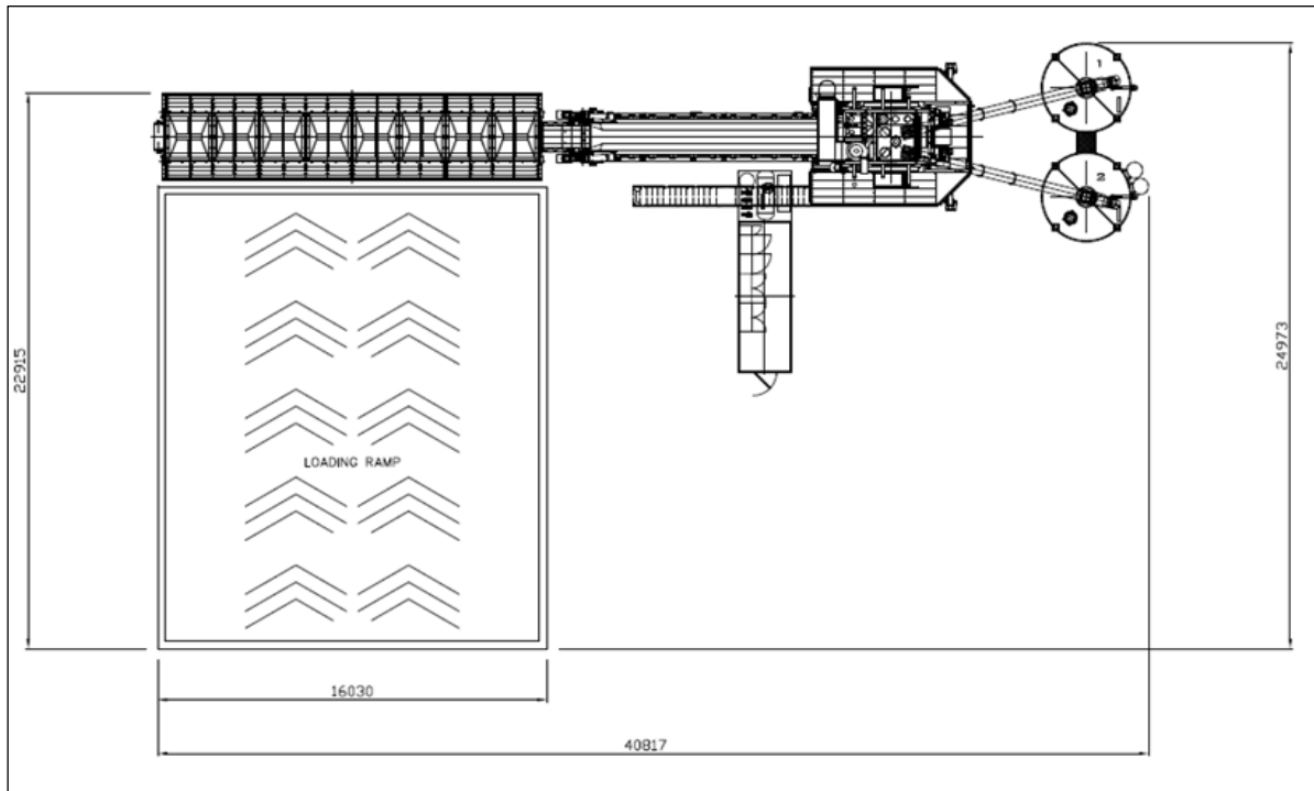
Figure 16-37: CRF Backfill Plant
