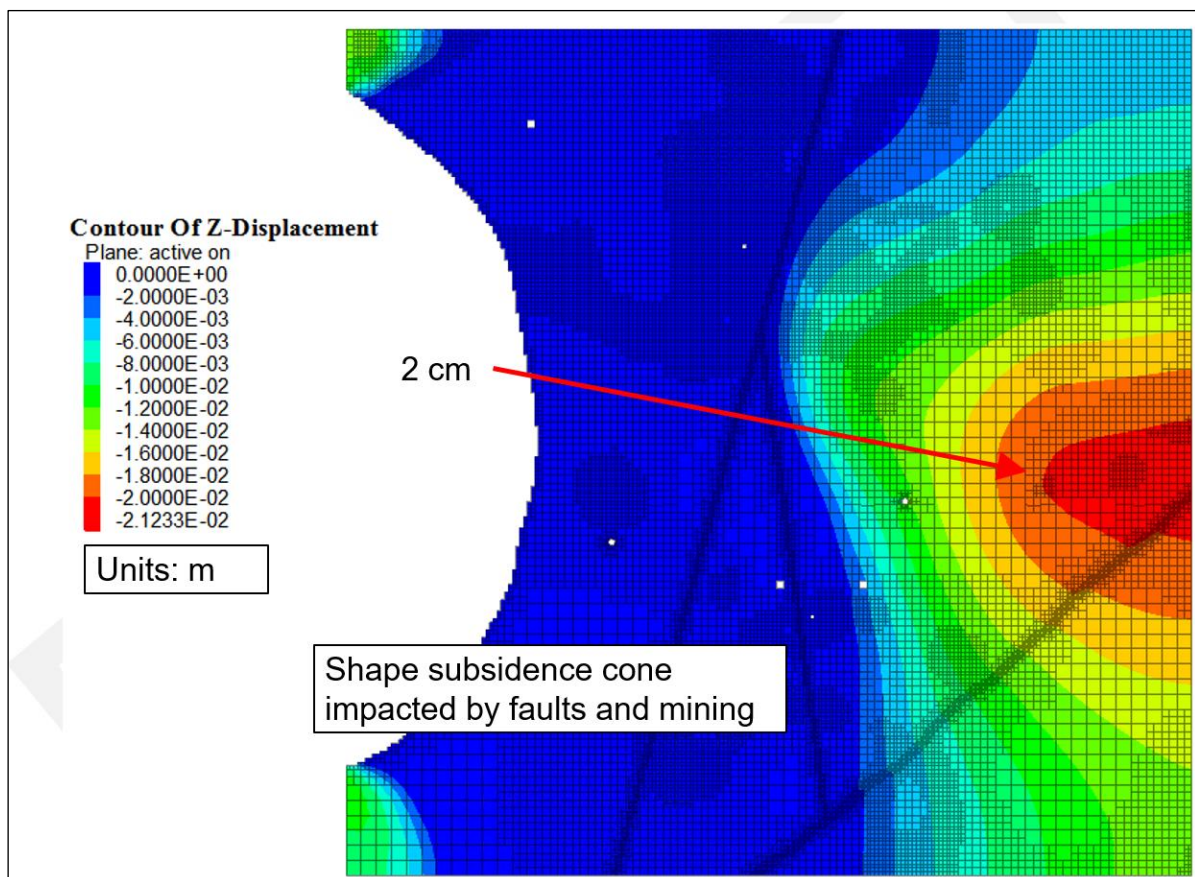
Figure 16-21: Plan View of Vertical Displacements Representing Surface Subsidence
