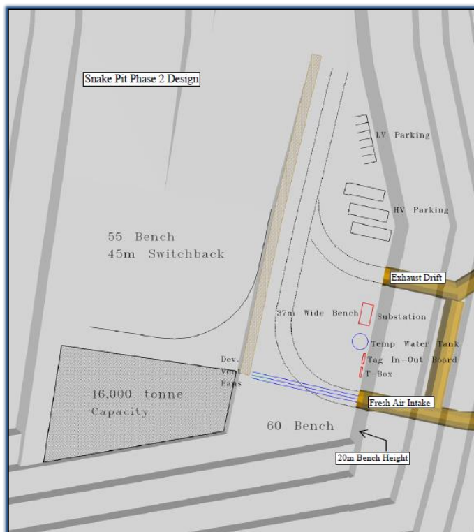
Figure 18-9: Layout for Ventilation Portals Area
