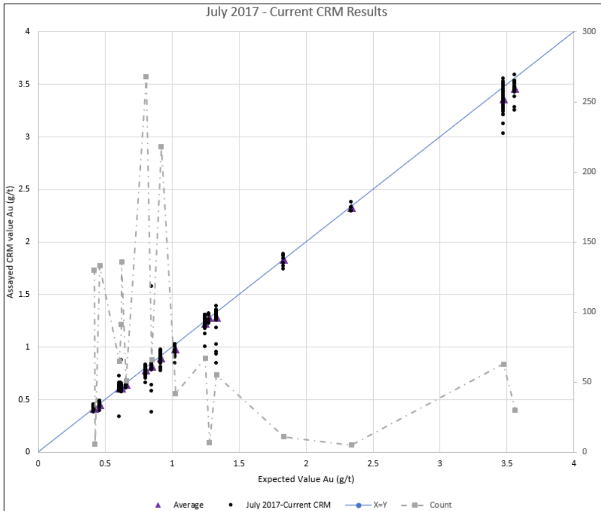
Figure 12-4: July 2017-Current CRM Analyses versus Expected Value <4 g/t (n=1,444)
