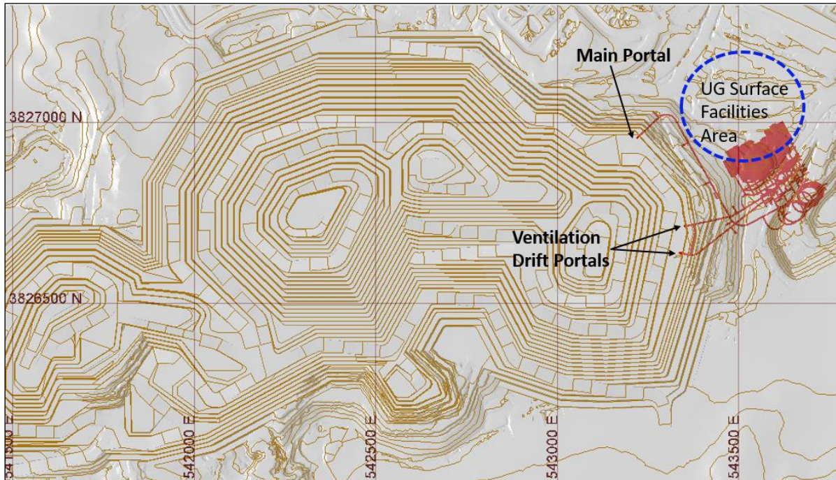
Figure 16-29: Underground Portal Location (shown in the OP coordinate system)
