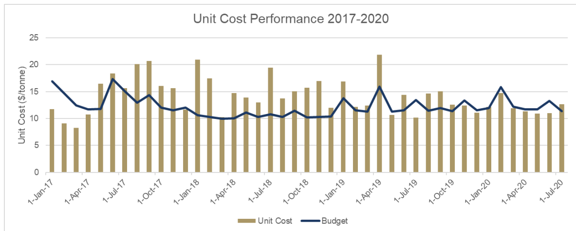
Figure 17-6: Process Unit Cost History Since Startup
