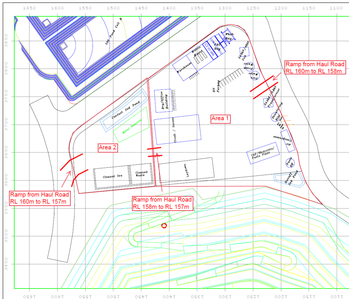
Figure 18-10: Underground Surface Infrastructure Detail
