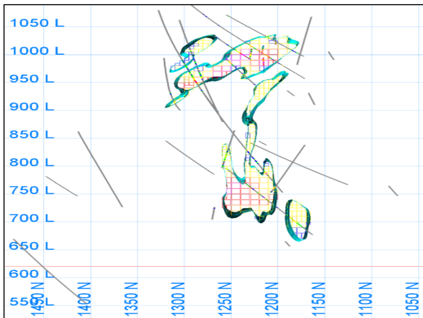
Figure 14-11: Representative Cross Section with Estimated Au Grades (Viewing E90°)
