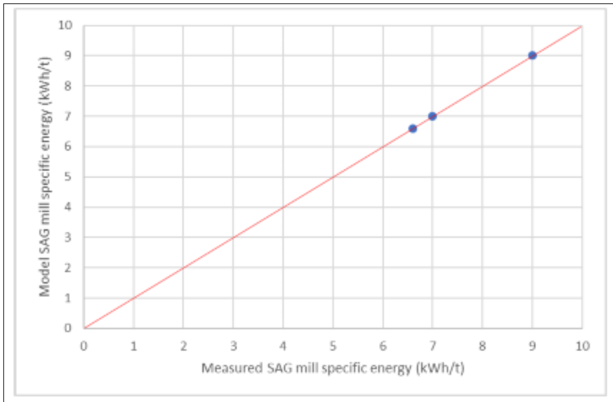
Figure 13-1 Modelled vs Measured SAG Specific Energy Values
