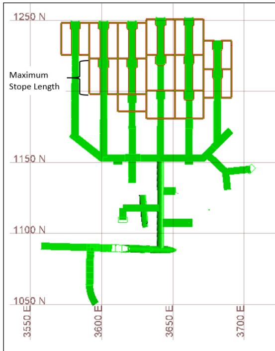
Figure 16-27: Level Cross Section of Stopes
