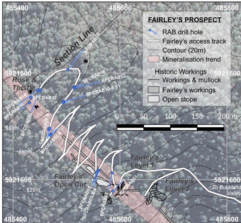
Figure 2: Plan of collars for the recent drilling at the Fairley's Prospect.
