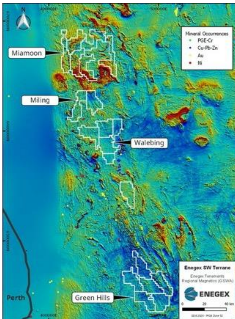
Figure 3 Eneget project areas over regional airborne magnetic data
