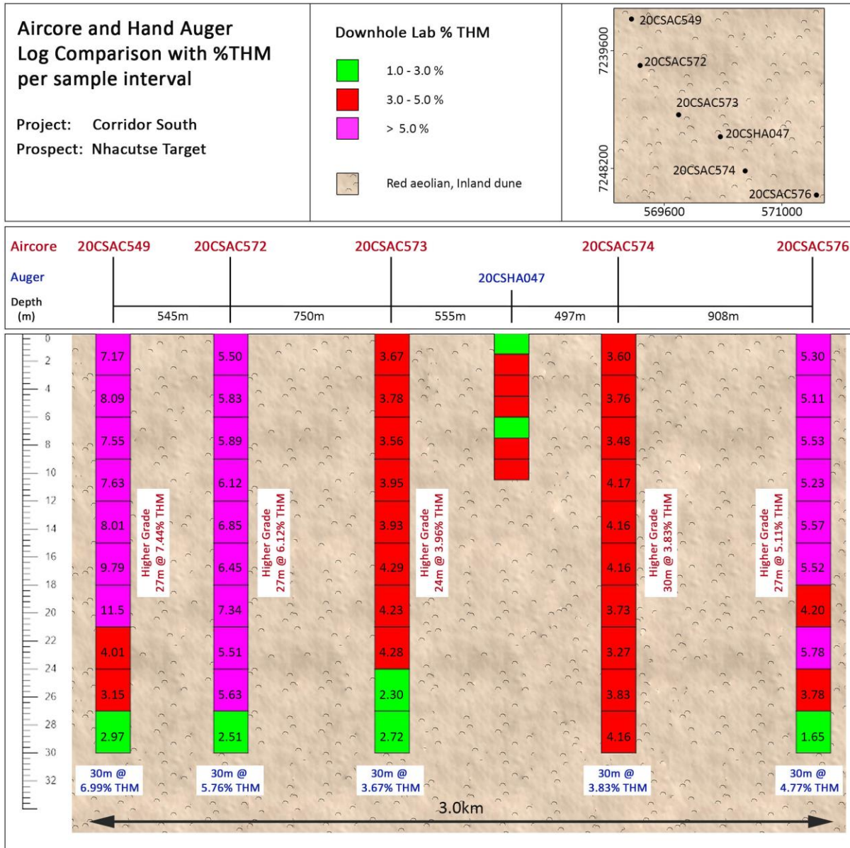
Figure 4: Cross section showing aircore and hand auger holes drilled between the towns of Nhatutse and Bungane, sections shows the link in grades, as well as the high THM grades in the Nhatutse High Grade zone. Section shows % THM results for each sample intersection, the average of the entire drillhole as well as where applicable a higher grade cut (using a lower cut-off of 3% THM) is shown. Note: The focus of this section is to show sample by sample downhole assays. Due to the vertical exaggeration required to do this, the surface profile is not shown.
