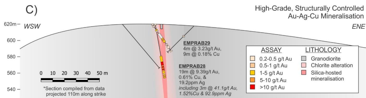
Figure 2: Cross-sections displaying preliminary geological interpretation of selected transects at Granite Flat, demonstrating the diversity and complexity of mineralisation styles encountered during drilling, including silica-sulphide mineralisation of breccia pipes (A), broad, low-grade Cu-Au mineralisation (B), and narrow, high-grade Au-Ag-Cu mineralisation (C). Drill results for historic drill holes DD92BO5, RC93BO22, RC93BO23 and DDH GF5 obtained from open file GSV reports (as reported in Dart ASX October 2020 ).
